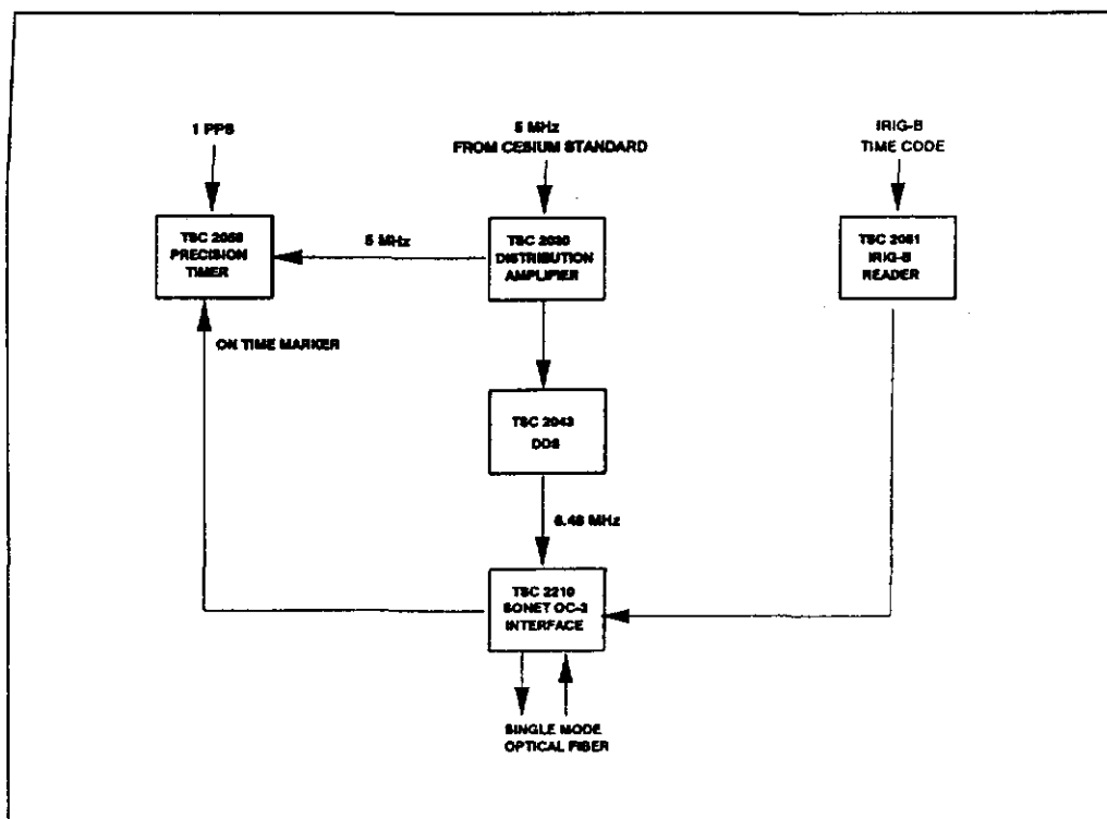
Figure 2. OTWTTT Master Unit Block Diagram
