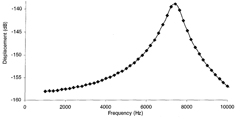
Fig. 4.4: Frequency response of a 7.4 kHz microresonator
