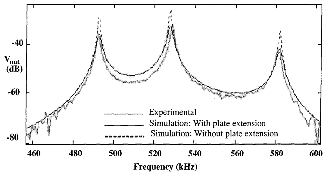
Fig. 4.2: AC transfer characteristics of the bandpass filter
