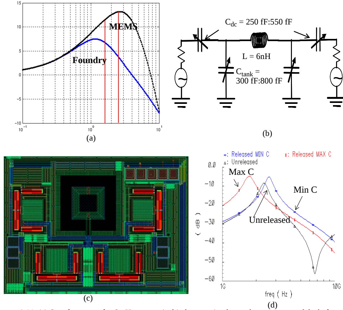
Figure 4-11. (a) Q vs frequency for 6-nH symmetrical inductor using lumped-parameter models, before and after release. (b) Design C schematic showing design values. (c) Layout of Design C filter. (d) S_{21} response of simulated filter before and after release, at both capacitor configurations.
