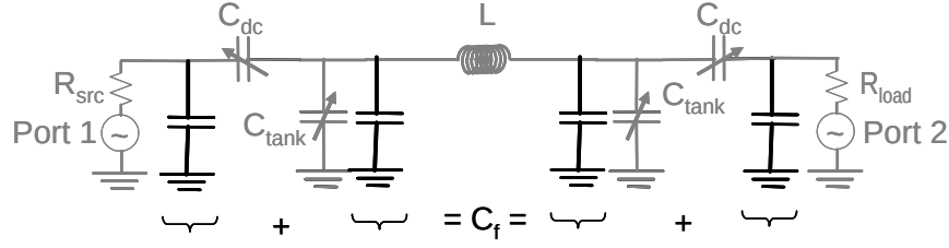
Figure 3-9. Filter schematic showing interconnect capacitances.
