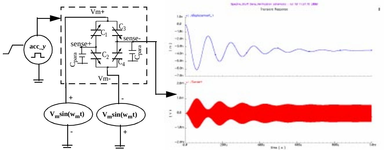
Fig. IV.3: Nominal Transient Simulation for Sensitivity Calculation
