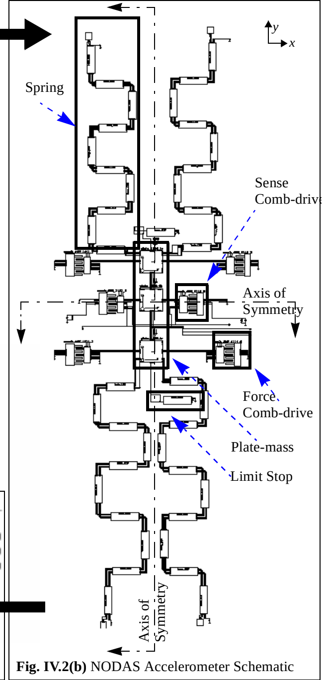
Fig. IV.2 CMOS Accelerometer Representations
