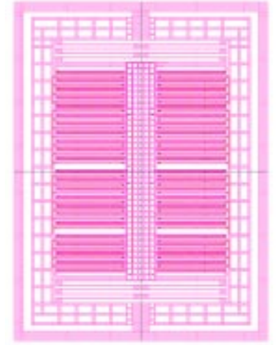
Gap= 1.5\mu\text{m} K_y=1.19\text{N/m} \omega_y=8.8\text{kHz}
