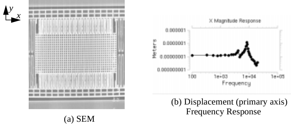
Fig. V.4: Range Accelerometer
