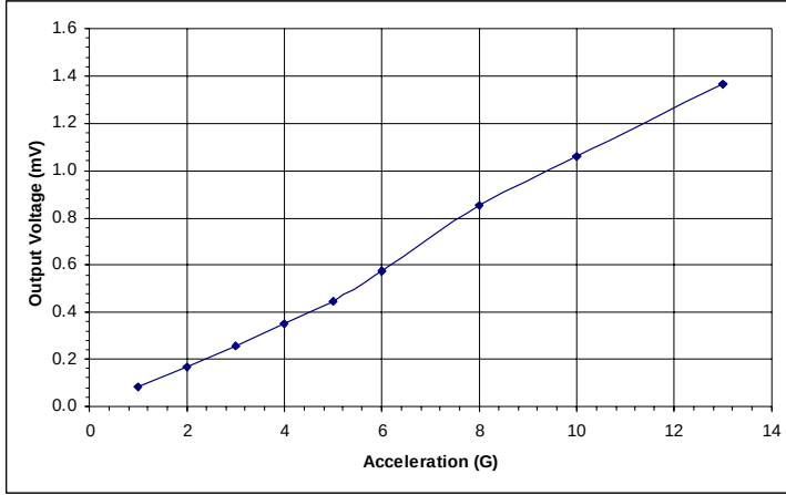
Fig. V.5: Dynamic Linearity of Range Accelerometer at 200Hz
