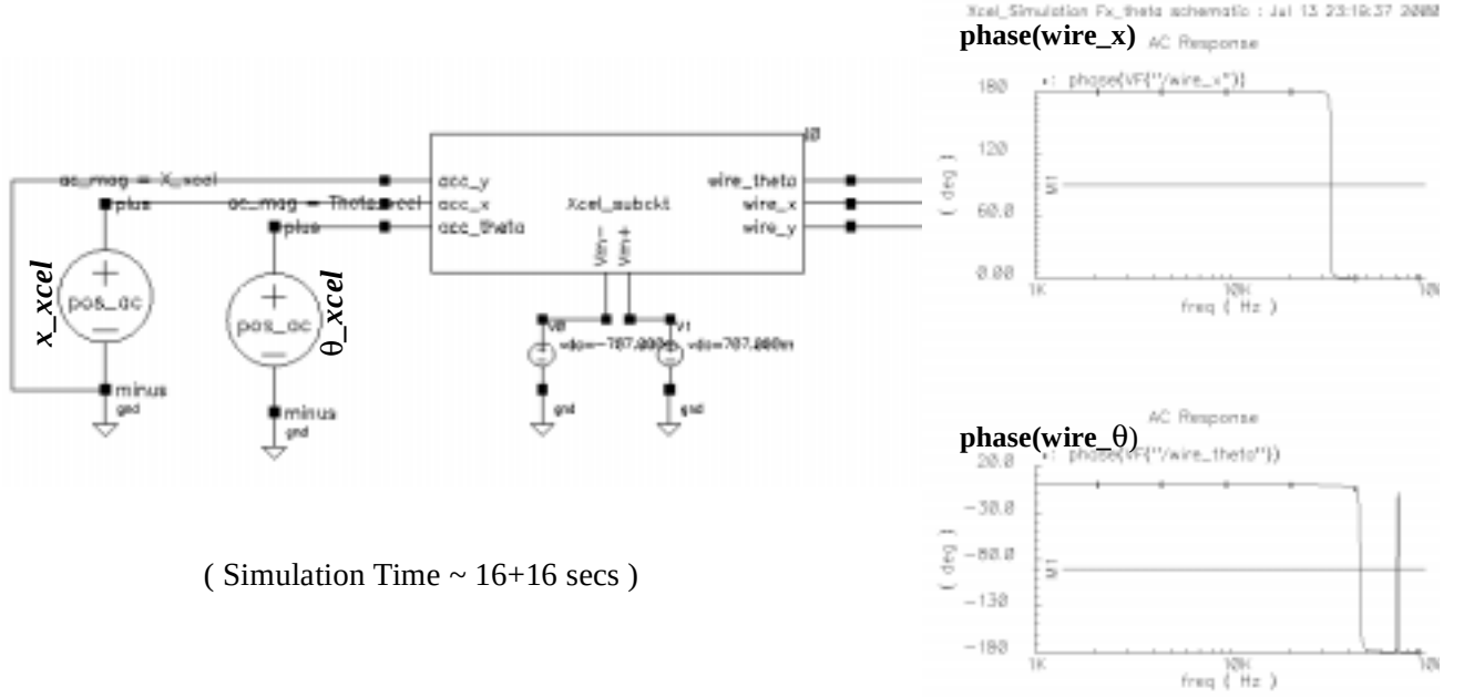
Fig. IV.6: Resonant Frequencies in x and \theta Directions
