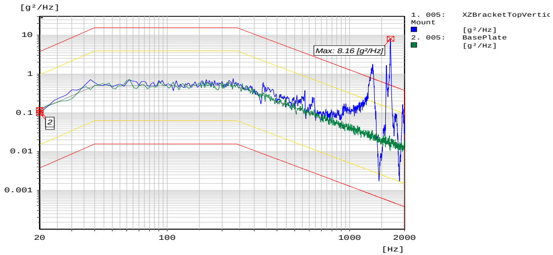
Figure 5. Random vibration, X/Z fixture, control (green), measurement (blue) in the direction of shaker motion
