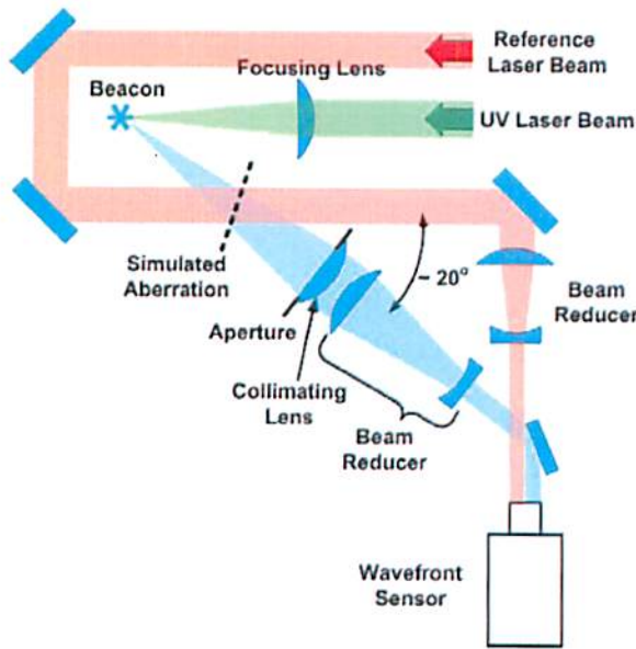
Fig. 11. Optical setup for stationary aberration measurements.
