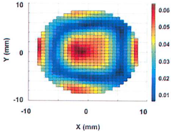
Figure 7. OPD_{rms} ( \mu\text{m} ) over aperture for typical baseline beacon wavefront measurement.
