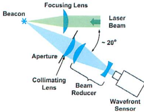
Figure 5. Optical setup for baseline beacon wavefront measurements.
