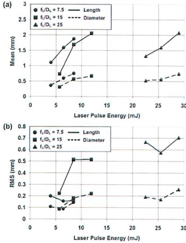
Figure 4. Spark dimensions from high-speed camera images
