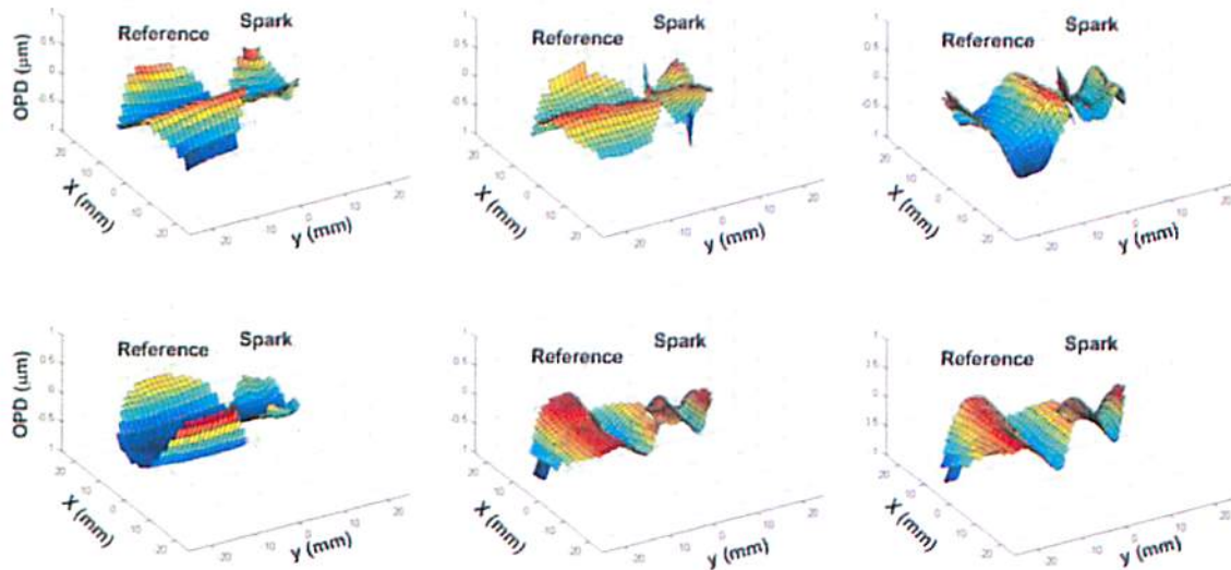
Fig. 12. Samples of wavefronts measured through 1/16^{\text{th}} -inch thick plexiglas plate. Spark wavefront is shown on the right of each image.
