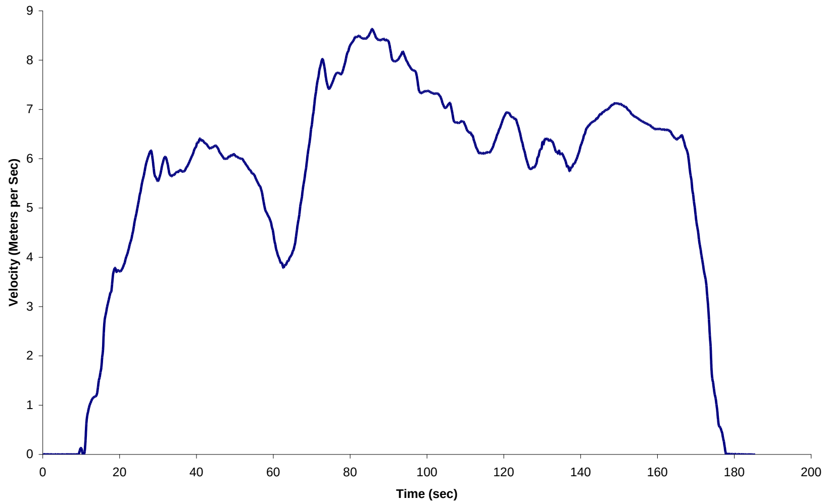
Figure 5-31 Velocity vs. Time plot for test scenario 4.
