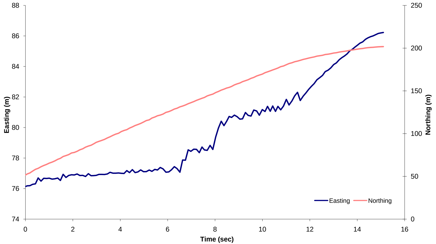
Figure 5-7 Easting and Northing vs. Time Plot for Test Scenario 1.
