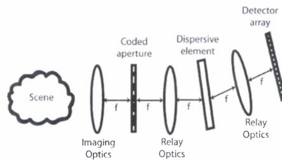
Figure 21: Schematic of an SD-CASSI. The imaging optics image the scene on to the coded aperture. The relay optics relay the image from the plane of the coded aperture to the detector through the dispersive element.
