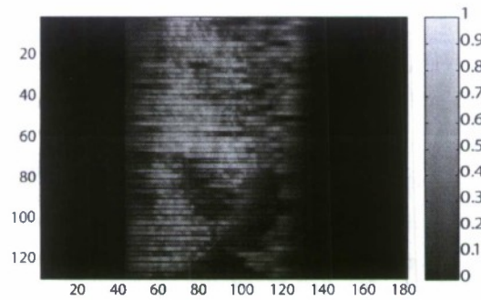
Figure 25: SD-CASSI detector measurement of the scene consisting of the two ping pong balls. Given the low linear dispersion of the prism, there is spatio-spectral overlap of the aperture code-modulated images of each ball.
