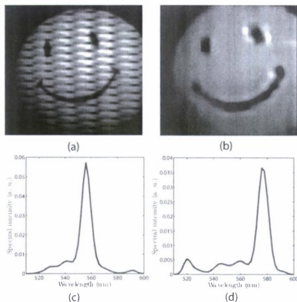
Figure 18: DD-CASSI experimental results from simple targets with narrow-band illumination. (a) Detector image recorded for illumination with a 10 nm FWHM bandpass centered at 560 nm. (b) Intensity image generated by summing the spectral information in the reconstruction for the 560 nm bandpass. (c) Spectral reconstruction at a particular spatial location for the 560 nm bandpass. (d) Spectral reconstruction at a particular spatial location for the 580 nm bandpass. The origin of the small peak near 520 nm is explained in the text.
