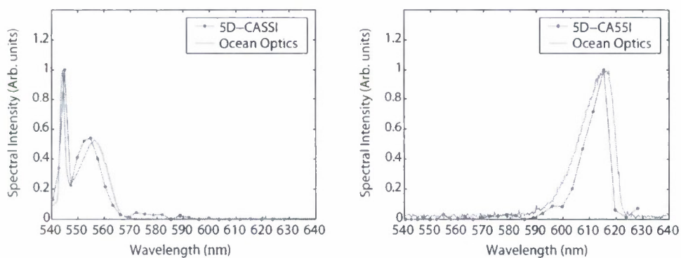
Figure 27: (a) SD-CASSI spectral intensity through a point on the ping pong ball illuminated with a 543 nm green laser and a white light source filtered by a 560 nm narrow band filter. (b) SD-CASSI spectral intensity through a point on the red ping pong ball illuminated with a white light source. Spectra from an Ocean Optics non-imaging reference spectrometer are shown for comparison.
