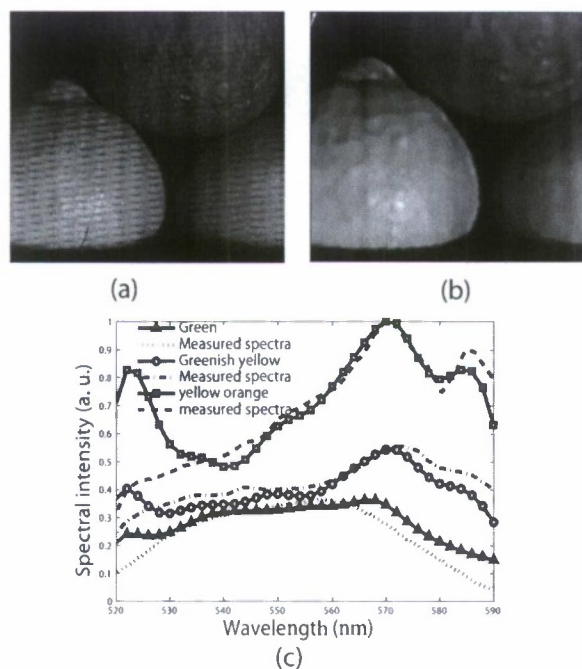
Figure 19: DD-CASSI experimental results from real-world objects under broadband (white) illumination. (a) Detector image recorded by the system. (b) Reconstructed intensity image of the scene. (c) Spectral reconstructions for spatial locations in the three regions.
