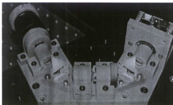
Figure 16: The DD-CASSI experimental prototype.
