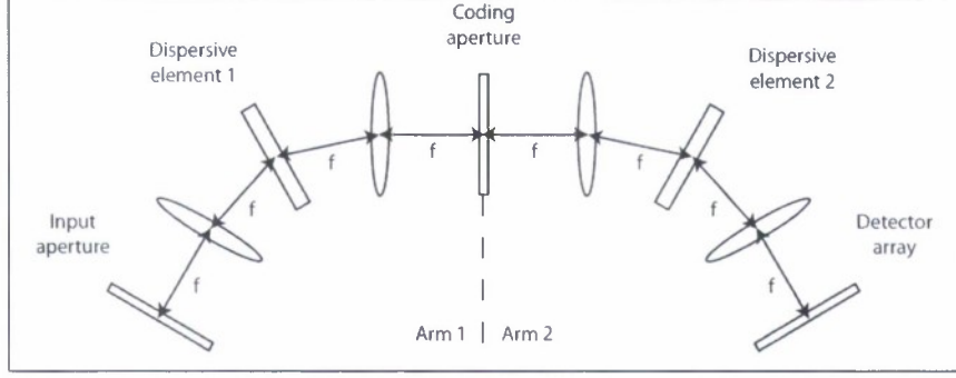
Figure 6: Schematic of the spectral imager.
