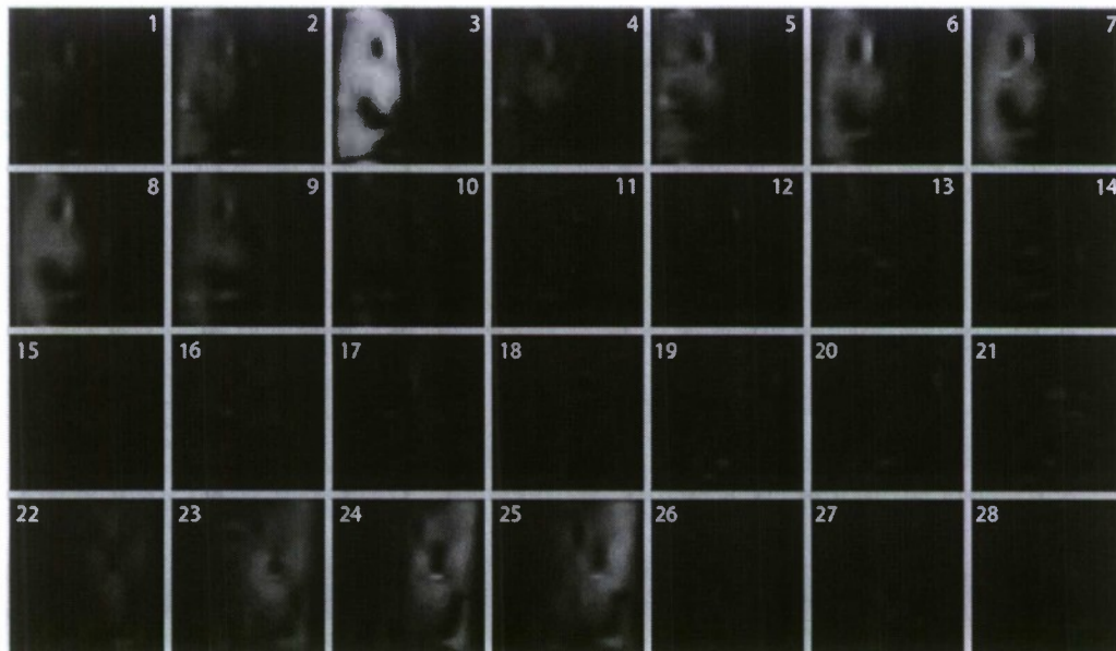
Figure 26: SD-CASSI estimated spatial content of the scene in each of 28 spectral channels between 540 nm and 640 nm. The green ball can be seen in channels 3, 4, 5, 6, 7 and 8, while the red ball can be seen in channels 23, 24 and 25.
