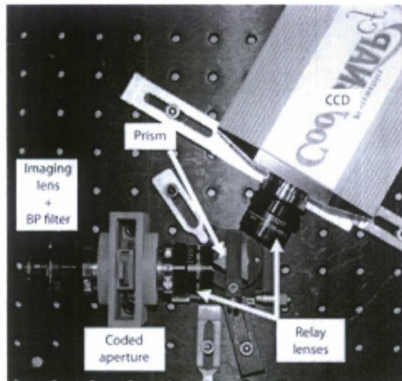
Figure 22: Experimental prototype of the SD-CASSI. The prototype consists of (i) a coded aperture, lithographically patterned on a chrome-on-quartz mask, (ii) three lenses from Schneider Optics Inc. with an f/\# of 1.4 and a focal length of 22.5 mm, (iii) an equilateral prism from Edmund Optics Inc. as a dispersive element, (iv) a monochrome charge-coupled device (CCD) detector from Photometrics with 1040 \times 1392 pixels that are 4.65 \mu\text{m} square each, and (v) a 500 - 620 \text{ nm} bandpass filter that is placed in front of the imaging lens to remove the impact of stray light on the experimental measurements.
