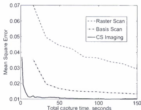
Figure 5: Average MSE for Raster Scan (RS), Basis Scan (BS), and Compressive Sampling (CS) single-pixel images as a function of the total image capture time T (real data).
