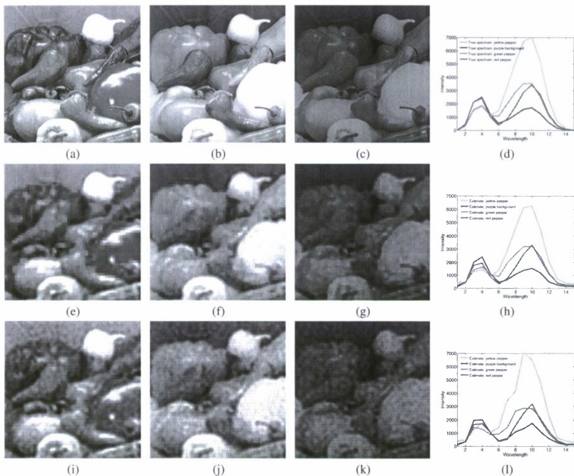
Figure 14: DD-CASSI reconstruction simulation results. (a) True intensity in 4 th spectral band. (b) True intensity in 8 th spectral band. (c) True intensity in 12 th spectral band. (d) Representative spectra from true spatio-spectral data cube. (e) Estimated intensity in 4 th spectral band, computed using reconstruction method described above with multiscale spatio-spectral regularization; MSE = 3.42 \cdot 10^{-2} . (f) Estimated intensity in 8 th spectral band, computed using reconstruction method described above with multiscale spatio-spectral regularization. (g) Estimated intensity in 12 th spectral band, computed using reconstruction method described above with multiscale spatio-spectral regularization. (h) Representative spectra from estimated spatio-spectral data cube, computed using reconstruction method described above with multiscale spatio-spectral regularization. (i) Estimated intensity in 4 th spectral band, computed using reconstruction method described above with no regularization; MSE = 4.61 \cdot 10^{-2} . (j) Estimated intensity in 8 th spectral band, computed using reconstruction method described above with no regularization. (k) Estimated intensity in 12 th spectral band, computed using reconstruction method described above with no regularization. (l) Representative spectra from estimated spatio-spectral data cube, computed using reconstruction method described above with no regularization.
