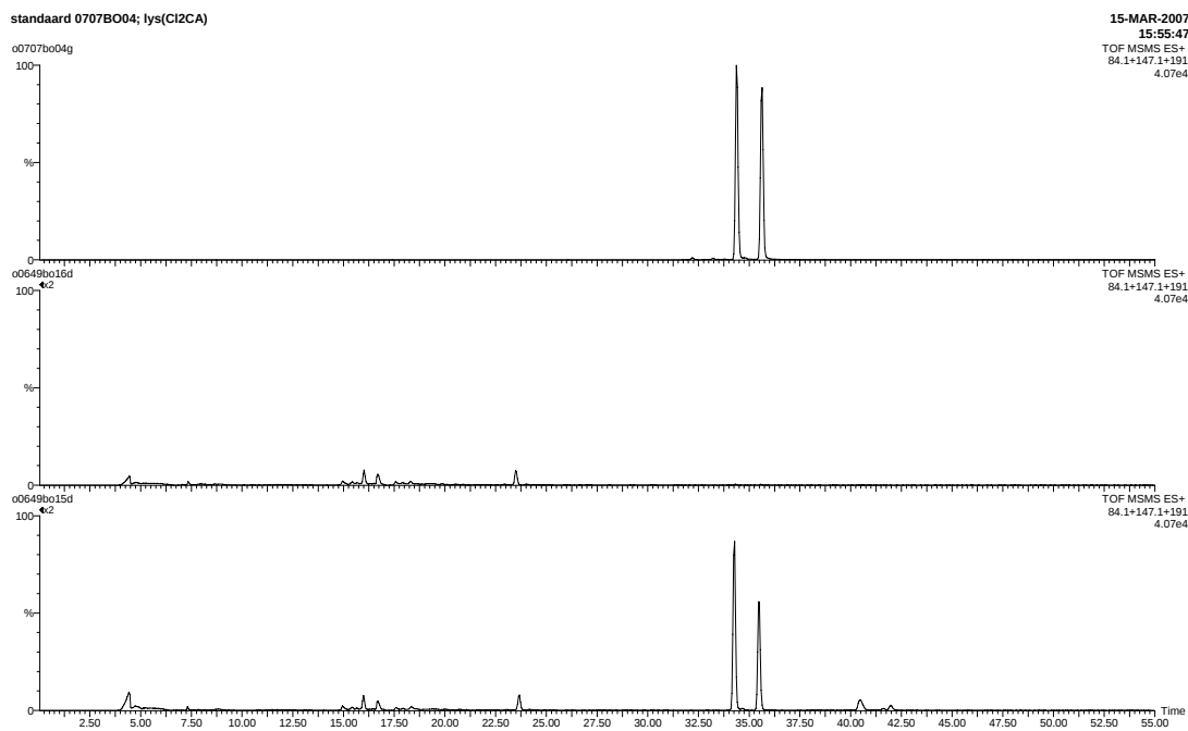
Figure 18. Ion chromatograms for \text{Cl}_2\text{CA} -modified lysine (transacylation adduct, both isomers) in a pronase digest of albumin isolated from human plasma that was incubated with synthetic \text{Cl}_2\text{CA} glucuronide. Upper trace, synthetic reference compounds; middle trace, blank plasma; exposed plasma.
