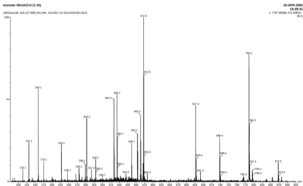
Figure 13. Tandem MS spectra of adduct of 3-PBA glucuronide with ASSAKQR, formed by the transacylation mechanism. Characteristic fragments: m/z 872.5 [ y_6'' + 196], 785.4 [ y_5'' + 196], 698.4 [ y_4'' + 196], 627.3 [ y_3'' + 196], 472.3 [ MH_2^{2+} ].
