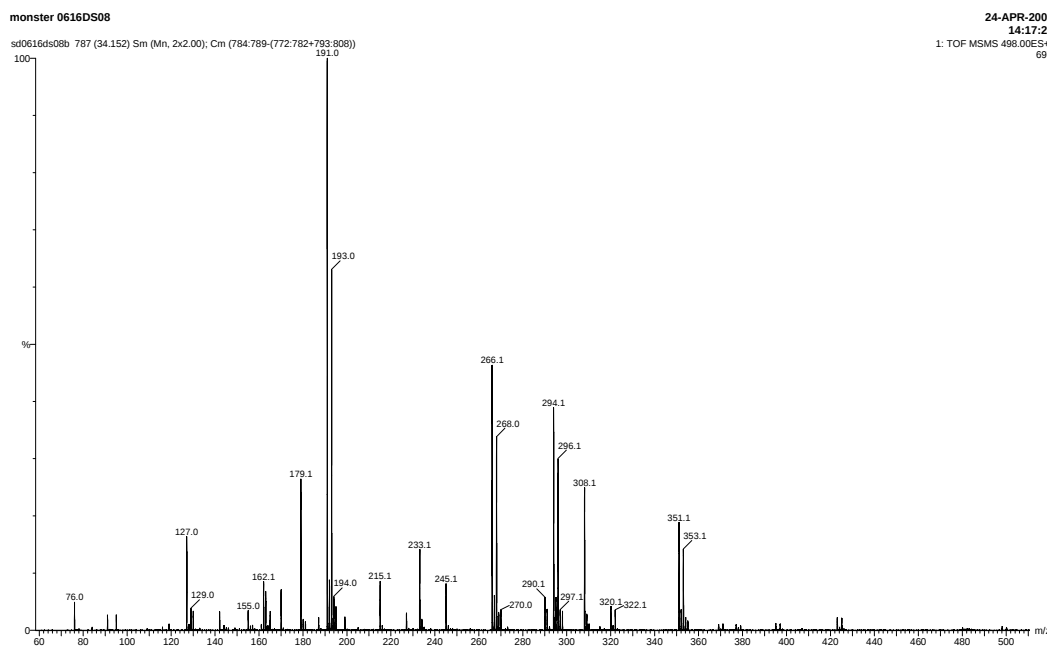
Figure 15. Tandem ES(+) MS spectrum of Cl_2CA -glucuronide to glutathione. Typical fragments for 498.0 [M + H]^+ : 351.1/353.1 [y_2' - H_2O] ; 294.1/296.1 [C(O)-NH-C=C-S-C(O)-dichlorovinyl-dimethylcyclopropyl]^+ ; 266.1/268.1 [H_3N-C=C-S-C(O)-dichlorovinyl-dimethylcyclopropyl]^+ ; 191.0/193.0, Cl_2CA fragment.
