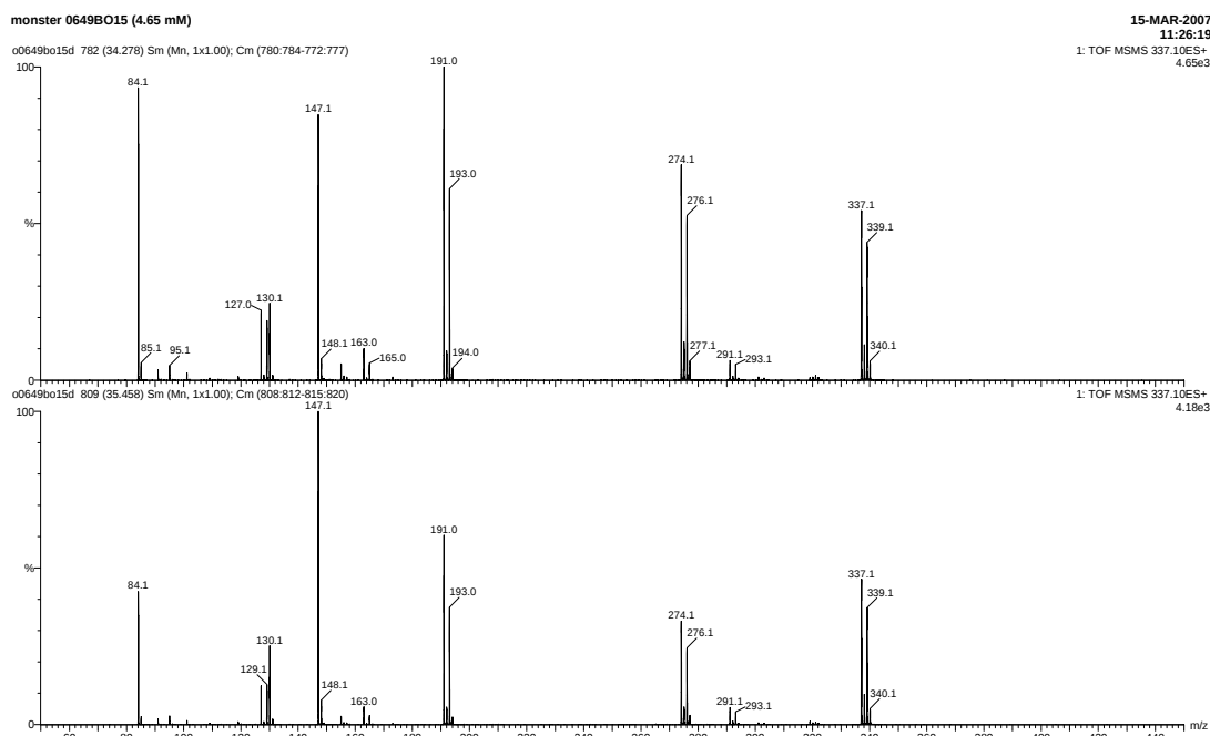
Figure 19. Tandem mass spectra of Cl 2 CA-lysine adduct in a pronase digest of albumin isolated from human plasma that was incubated with Cl 2 CA glucuronide. Upper trace: fast eluting isomer. Lower trace: slow eluting isomer (see Figure 18).
