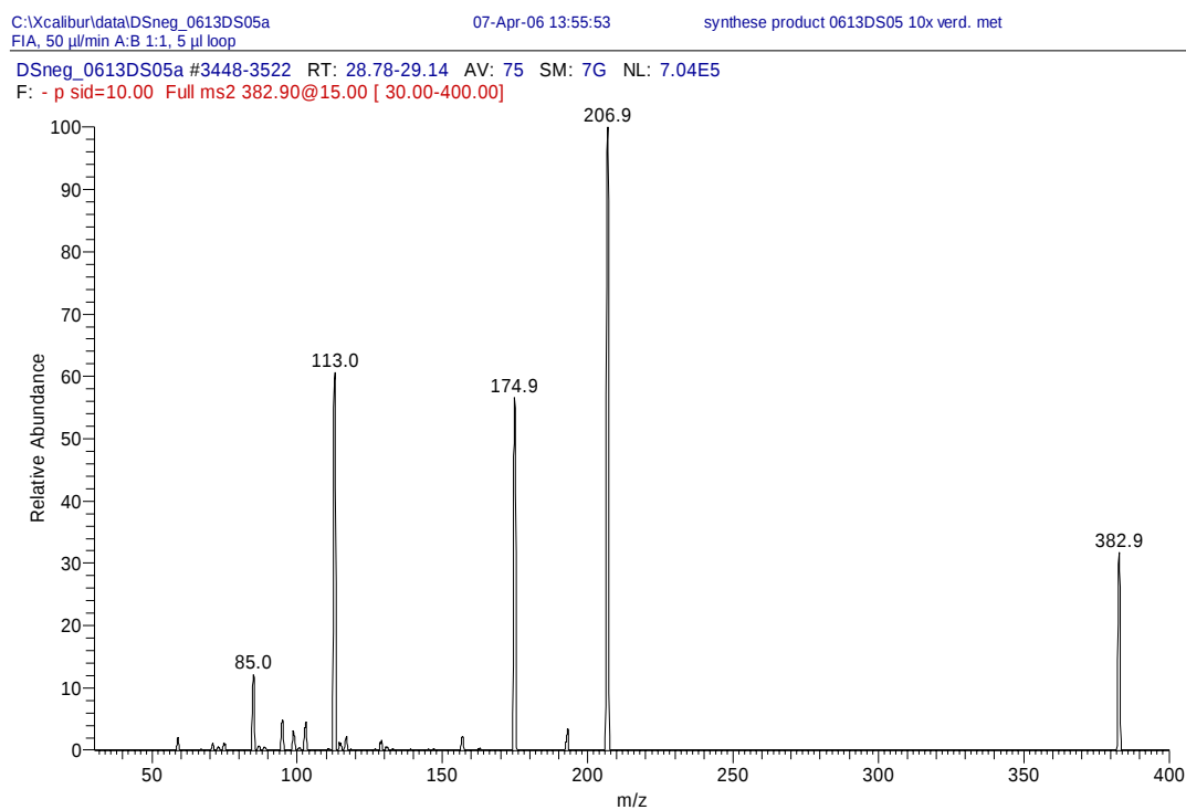
Figure 6. Mass spectrum (upper trace) of Cl 2 CA glucuronide; 382.9 [M-H] - , 428.9 [M+HCOO] - , 768.9 [2M-H] - . Tandem MS spectrum of Cl 2 CA glucuronide (lower trace): 206.9 [Cl 2 CA] - , 174.9 [382.9 – Cl 2 CA] - , 113.0 [174.9 – H 2 O – CO 2 ].
