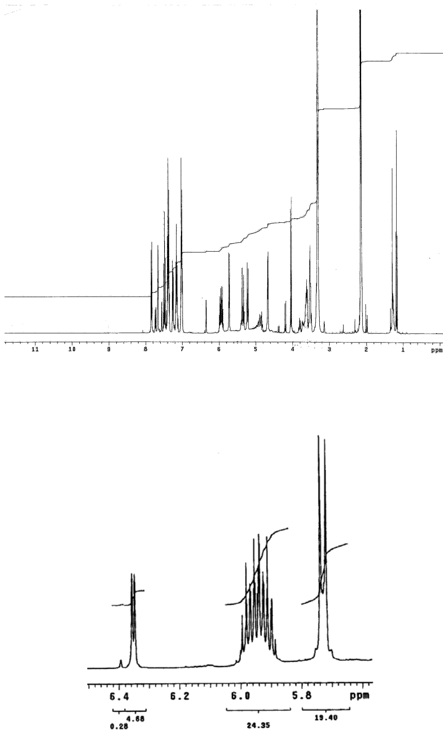
Figure 1A. 1 H-NMR spectrum of anomeric mixture of allyl 1-O-(3-phenoxybenzoyl)-D-glucopyranuronate (2). Upper panel: entire 400 MHz 1 H-NMR spectrum. Lower panel: part of the spectrum, showing the H1-α around 6.4 and H1-β around 5.7. The multiplet around 5.9 – 6.0 is part of the allyl group.
