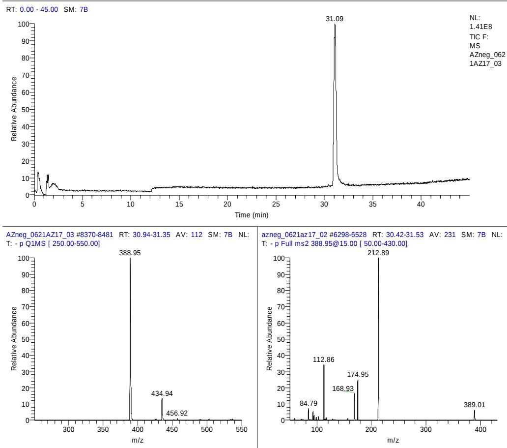
Figure 4. LC-MS and LC tandem MS spectra of 3-PBA \beta -glucuronide. The upper panel represents the total ion current (ES-). The lower, left panel is the corresponding mass spectrum; 389 [M-H] - ; 434.9 [M + HCOO] - . The lower, right panel represents the tandem MS spectrum; 212.9 [3-PBA] - , 174.9 [389 - 3-PBA] - , 168.9 [3-PBA - CO 2 ] - , 112.8 [174.9 - H 2 O - CO 2 ] - .
