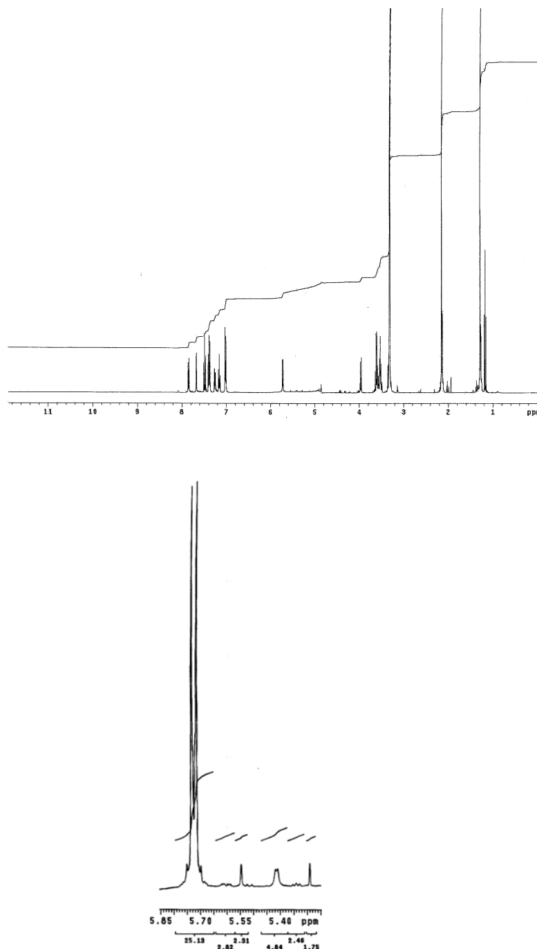
Figure 2A. ^1\text{H} -NMR spectrum of anomeric mixture of 1-O-(3 phenoxy-benzoyl)-D-glucopyranuronate (3; 3-PBA-glucuronide). Upper panel: entire ^1\text{H} -NMR spectrum. Lower panel: part of the ^1\text{H} -NMR spectrum, showing the characteristic doublet of \text{H1-}\beta around 5.7.
