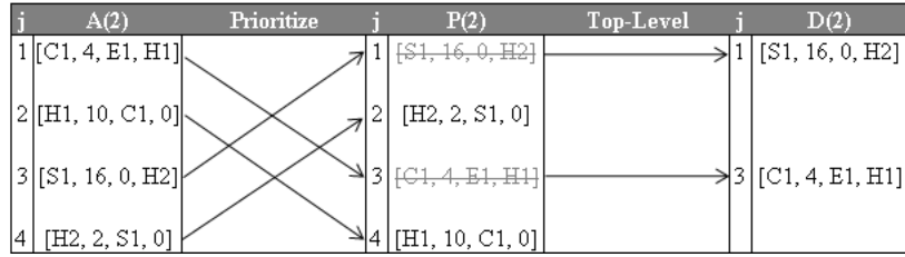
Figure 4.7 Prioritize Subroutine (t = 2 “Tuesday”, n = 0)
