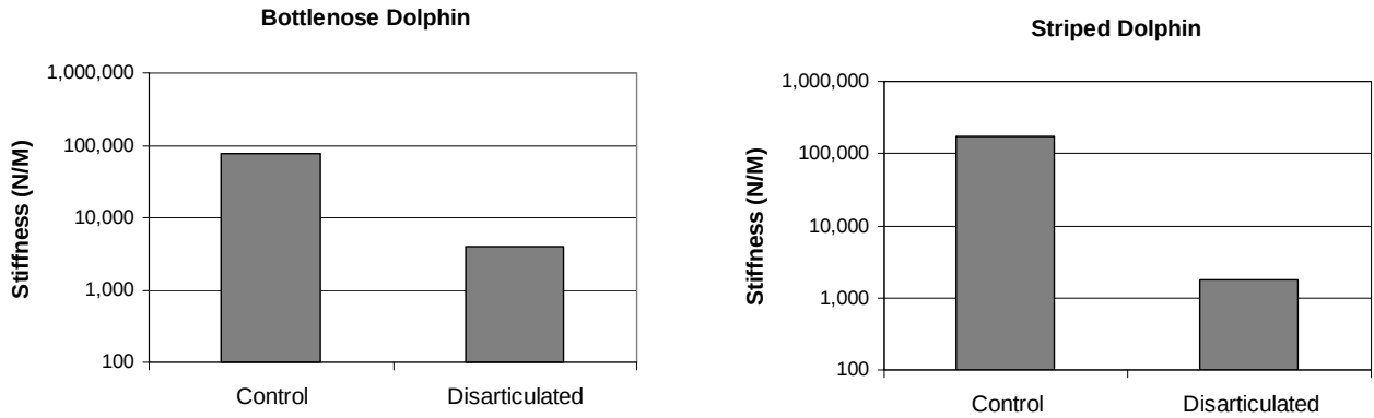
Figure 3. Effect of disrupting ossicular chain on middle-ear stiffness
