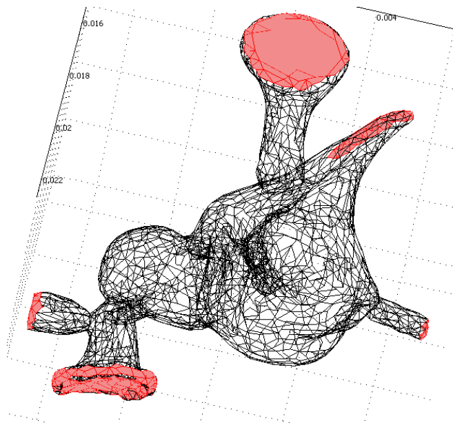
Figure 6. Tursiops middle ear finite-element model mesh
