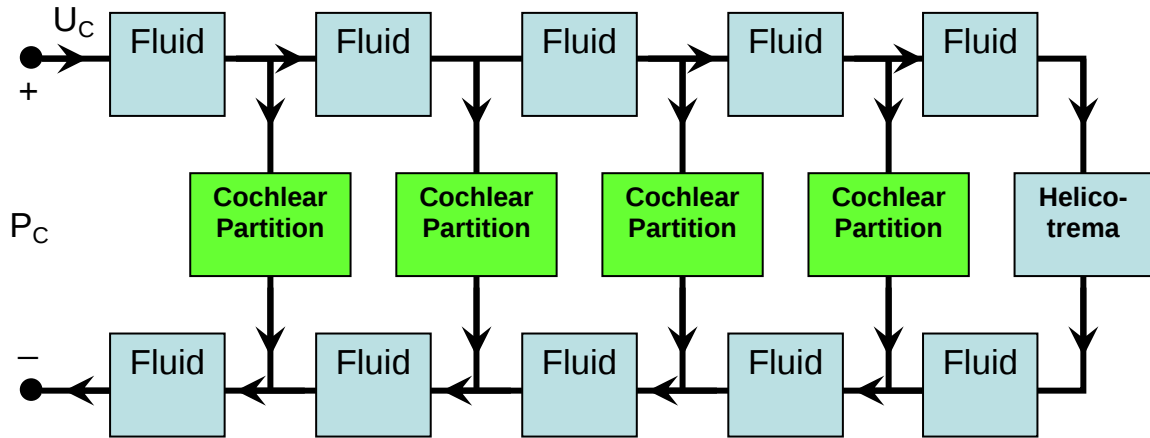
Figure 11. Cochlear finite-difference model
