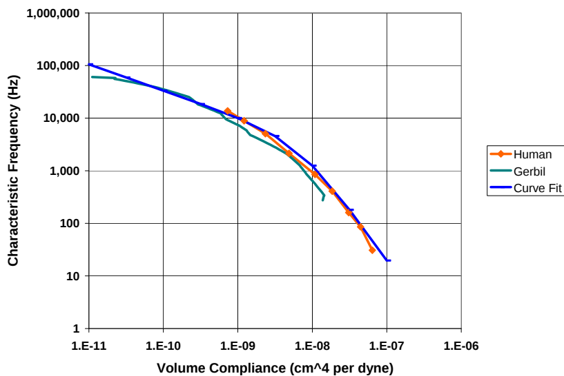
Figure 10. Compliance-frequency map.
