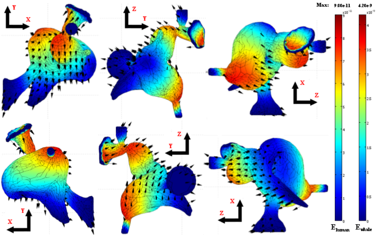
Figure 7. Predicted displacements from the dolphin FEM model for a force applied to the stapes.
