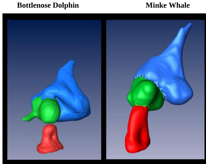
Figure 5. 3D middle ear reconstructions for bottlenose dolphin and minke whale. Note that the boney process of the minke malleus (blue) is longer and thinner than that in the dolphin, which suggests that the minke middle ear is much more compliant than the dolphin middle ear.
