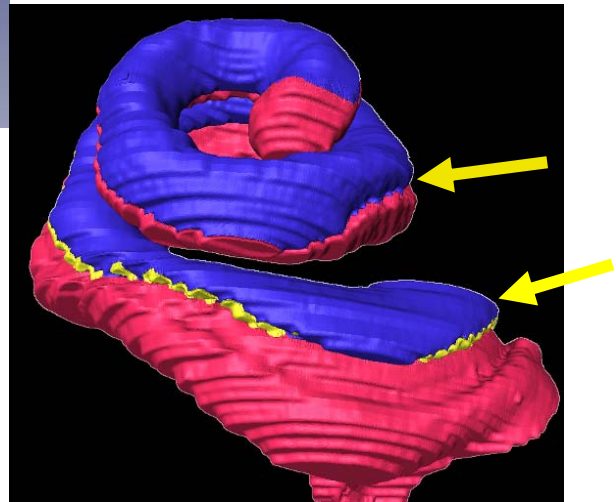
Figure 2. Three-dimensional reconstruction of the scalae and basilar membrane from celloidin histology of a minke whale temporal bone.
