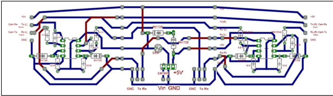
Figure 15. RS-232 to TTL Signal Conversion Circuit (See diagram in Appendix F)
