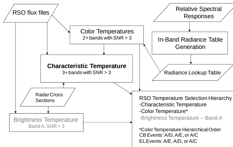
Figure 1: Measured fluxes from RSO candidates are used to derive the object temperature. For each RSO, the color temperature and the radar cross section are used as initial estimates (“seed values”) for the characteristic temperature determination algorithm. The final output to the catalog depends upon the number of bands for which data is available.
