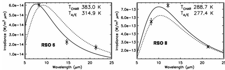
Figure 6: Characteristic Fits to Data. Three bands fit, Q < 0.1 .
