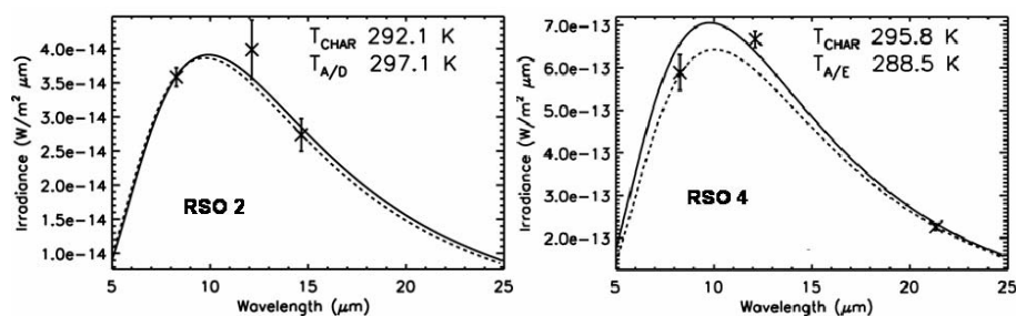
Figure 5: Characteristic Fits to Data. Three bands fit, Q > 0.1 .
