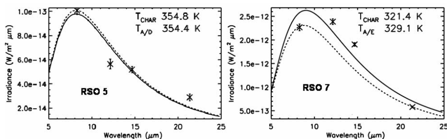
Figure 4: Characteristic Fits to Data. Four bands fit, Q < 0.1 .
