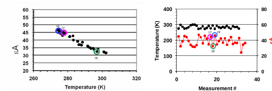
Figure 9: (left) \epsilon A versus T_{\text{color}} (A/D) for an EM12 observation of the Hubble Space Telescope. (right) Temporal evolution of T_{\text{color}} (upper curve, black points, left hand axis) and \epsilon A (lower curve, red points, right hand axis). Measurements were slightly irregular but average \sim 3 seconds apart.
