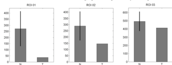
Fig. 2: Comparison of the tract count between normals (N) and the TBI subject (T) along pathways shown in Fig. 1 at FA>0.2 . The effect sizes for the connectivity reduction are: 1.66, 1.24 and 0.68 respectively, which are significant large effects.
