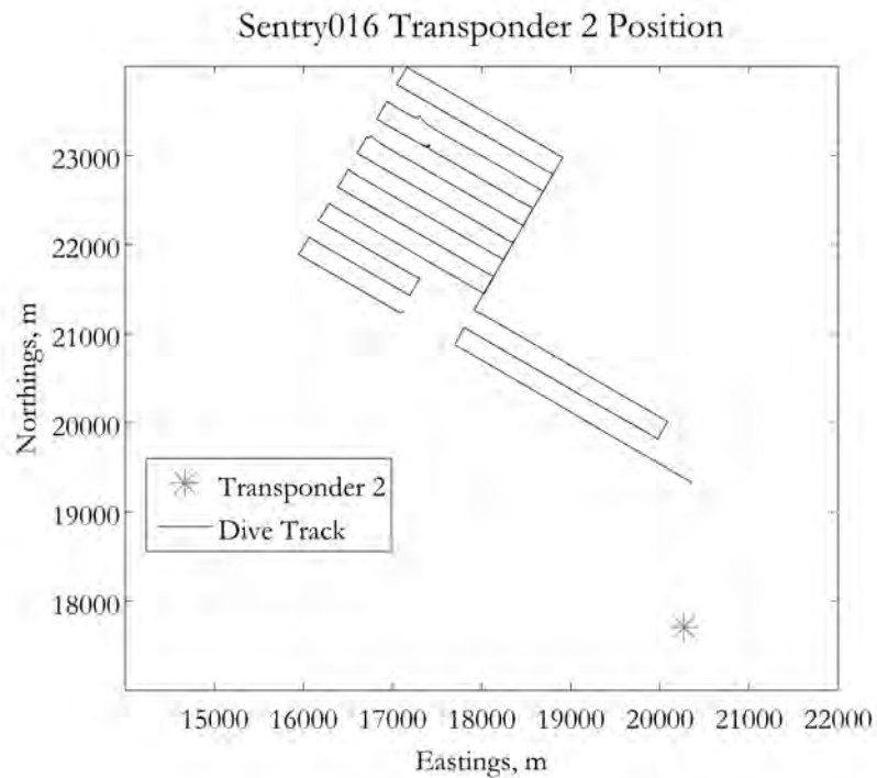
Figure 7-59: Sentry016 tracklines and Transponder 2 location.
