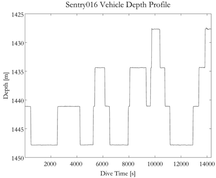
Figure 5-1: Sentry016 vehicle depth profile.
