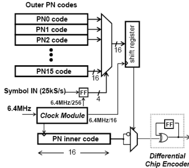
Figure 25: Transmitter Block
