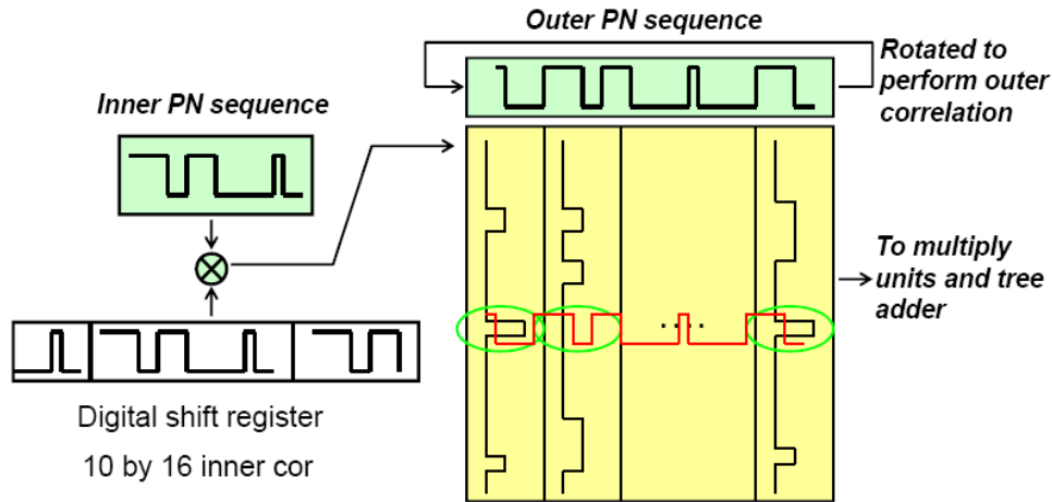
Figure 23: Correlator Peak detection
