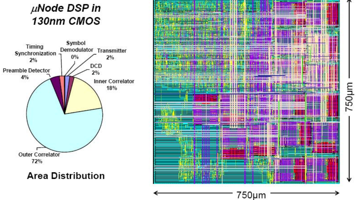
Figure 37: \mu Node digital signal process 130 nm CMOS layout
