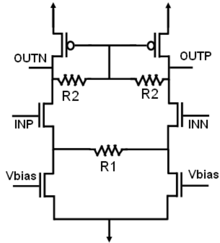
Figure 31: VGA basic cell
