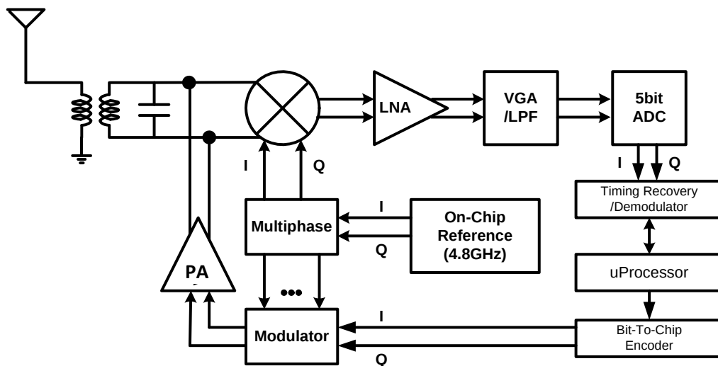
Figure 27: Differential RF front-end \mu Node
