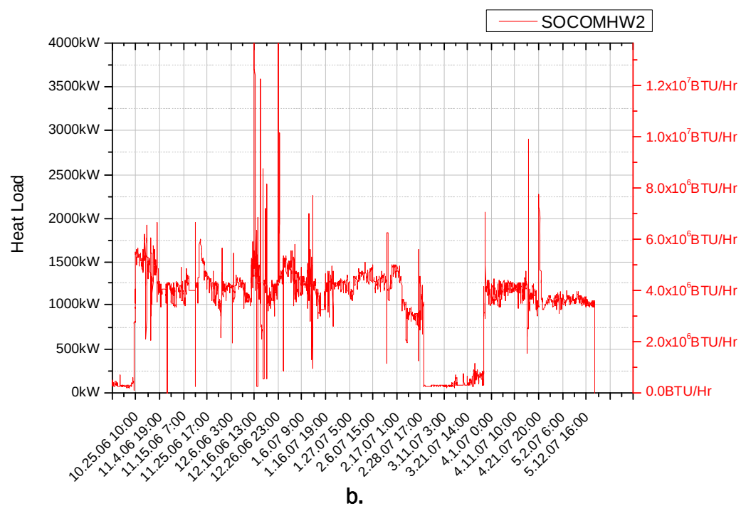
Figure 2.14. Calculated load curves for the SOCOM Plant: (a) Zone 1 and (b) Zone 2.
