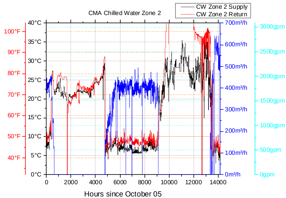
Figure 2.29. Metered chilled water energy data from CMA Plant: (a) Zone 1 and (b) Zone 2.
