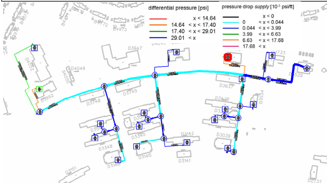
Figure 5.4. DH system for CMA D-Area, Control Zone 3.
