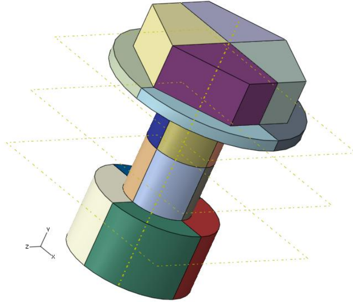
Figure 10: Pin partitions
