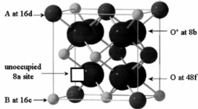
Figure 4: Schematic of the partial unit cell of the pyrochlore structure [[28]].
