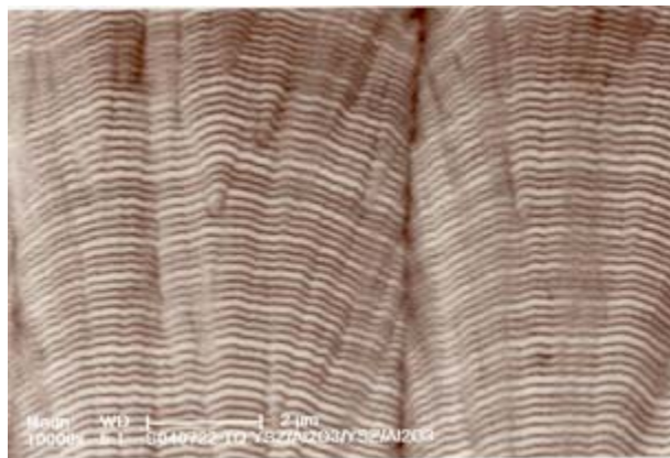
Figure 7: Multiple layered 8YSZ/ \text{Al}_2\text{O}_3 structure with increased hemispherical reflectance.
