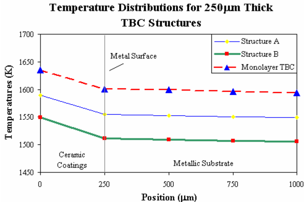
Figure 12: Computed temperature distributions for 250 \mu m thick multiple layered coating compared with mono-layered coating. Design structure A: multiple layers on the top of the single layer; Design structure B: single layer on the top of multiple layers.
