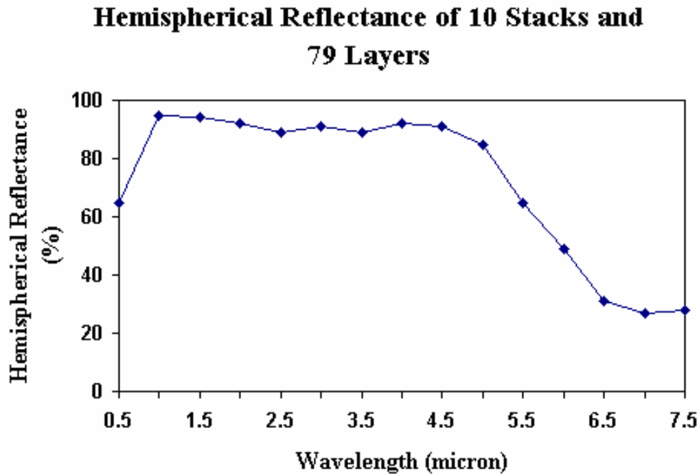
Figure 10: Calculated hemispherical reflectance of 10 stacks with 79 layers.
