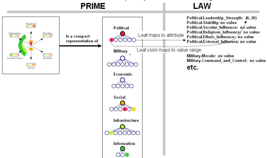
Figure 23: Conceptual view of mapping between PRIME's starbursts and LAW's attribute-value pairs
