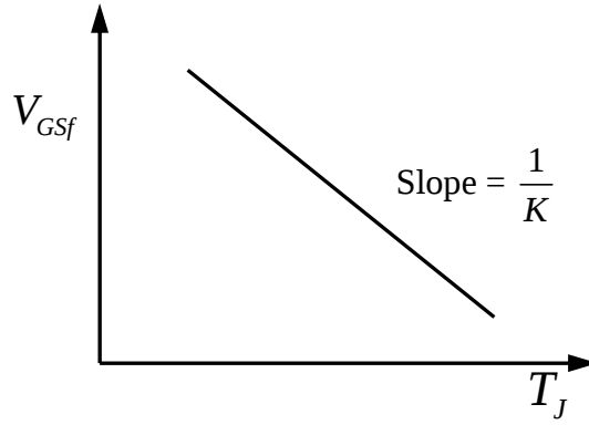
Figure 14. Calibration Curve.
