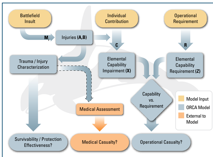
Figure 2 ORCA Methodology
