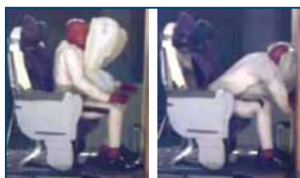
100 ms (left) vs. 140 ms (right). The AmSafe Aviation Airbag functions during a 16g, 180ms impact. It is installed in the front row economy behind a bulkhead.
