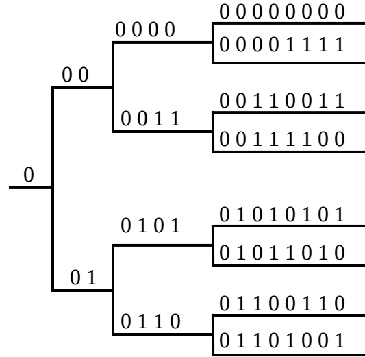
Figure 6. Variable length orthogonal sequences before mapping. (From: [2]).
