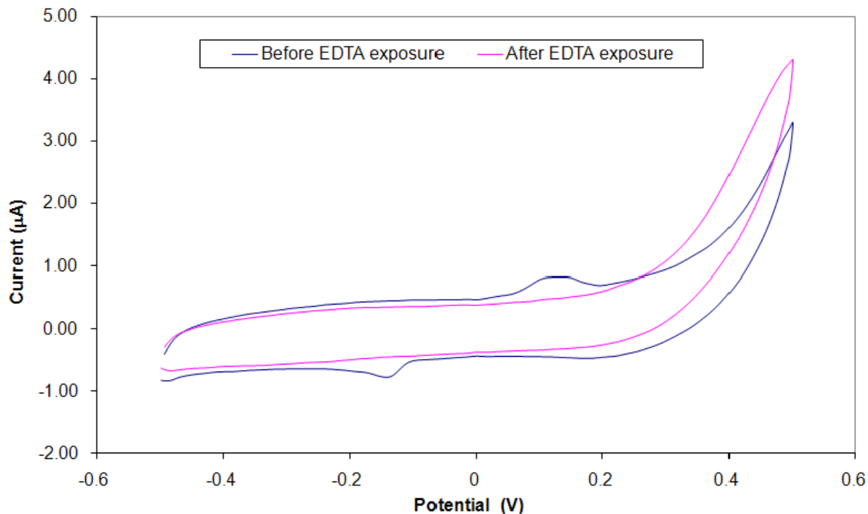
Figure 3. Cyclic Voltammetry of Superoxide Dismutase on Gold Electrode as Influenced by 0.1 mM EDTA.
