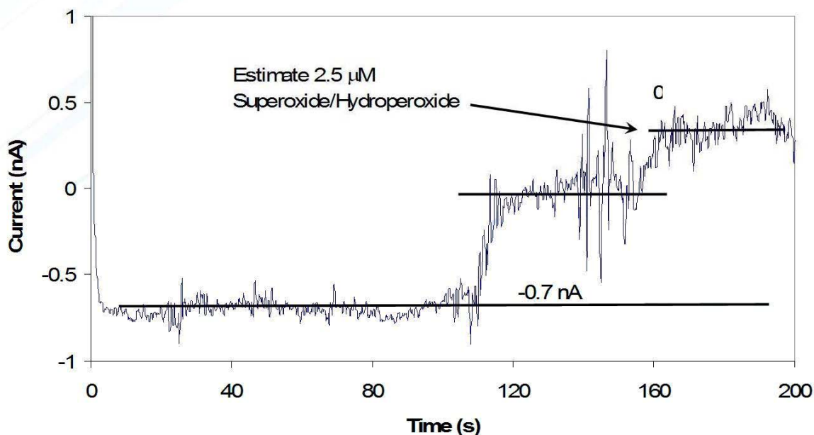
Figure 2. Response of Superoxide Dismutase Sensor to O_2^{\bullet -}/HO_2^{\bullet} Produced with Xanthine Oxidase and Acetaldehyde. Xanthine oxidase solution mixed stepwise ( \sim 100 \text{ s} and \sim 160 \text{ s} ) with buffer in which electrode was suspended.
