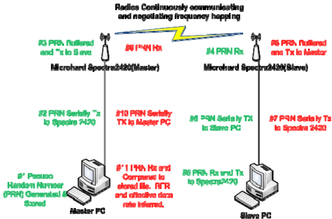
Figure 8. Python Serial Test Program Diagram
