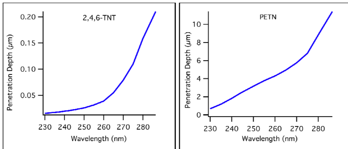
Figure 27. Calculated penetration depth of the UV Raman signal for the phenyl ring stretch of 2,4,6-TNT (left) and symmetric NO 2 stretch of PETN (right).
