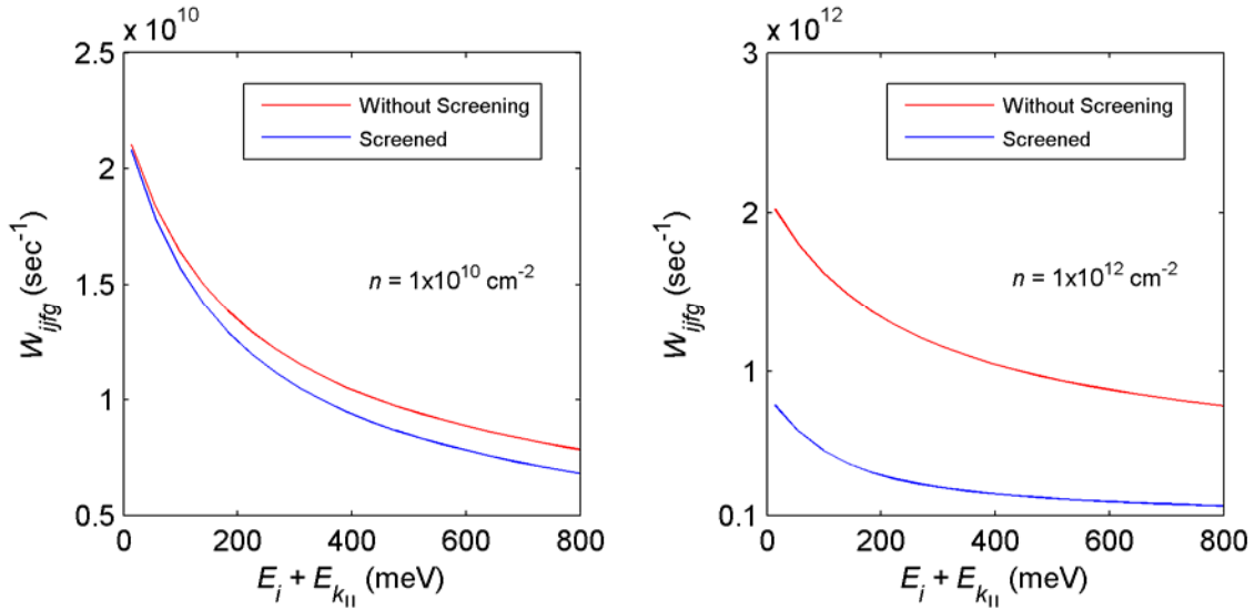
Figure III.B.3. Electron-electron scattering rate as a function of total energy at T = 300 \text{ K} , with and without including screening, for subband populations of (a) 1 \times 10^{10} and (b) 1 \times 10^{12} \text{ cm}^{-2} .
