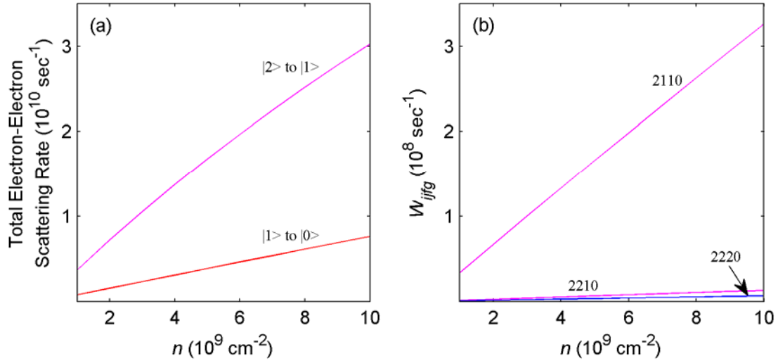
Figure VI.A.3. Scattering rates for the 4.3 THz step quantum well for T_{\text{electron}} = 100 \text{ K} . (a) The total electron-electron scattering rates for the 2 to 1 and the 1 to 0 transitions, based on the processes for the simplified rate equation analysis, as a function of initial state populations. (b) The mean electron-electron scattering rates as a function of initial state populations for T_{\text{electron}} = 100 \text{ K} , for some additional scattering processes for the 2 to 1 transition that are not within the framework of the simplified rate equation analysis.
