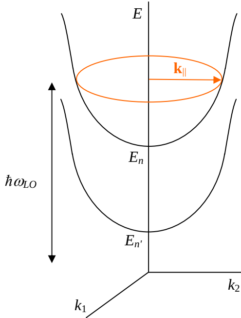
Figure III.A.5. LO-phonon emission case 1a, E_n - E_{n'} < \hbar\omega_{LO} and the electron does not have sufficient in-plane kinetic energy, forbidden transition.
