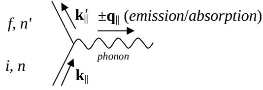
Figure III.A.3. Feynman diagram for electron-phonon scattering.
