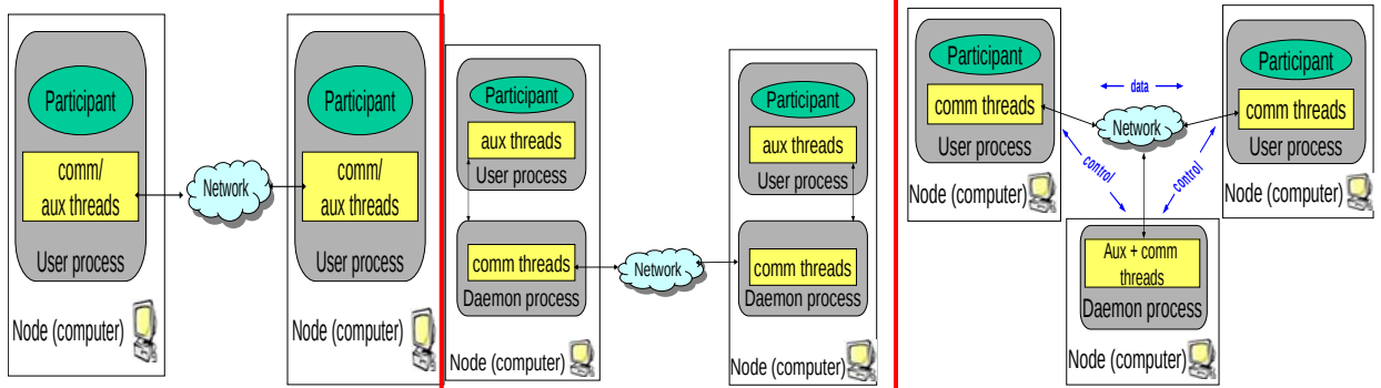
DDS1 - Decentralized Architecture
