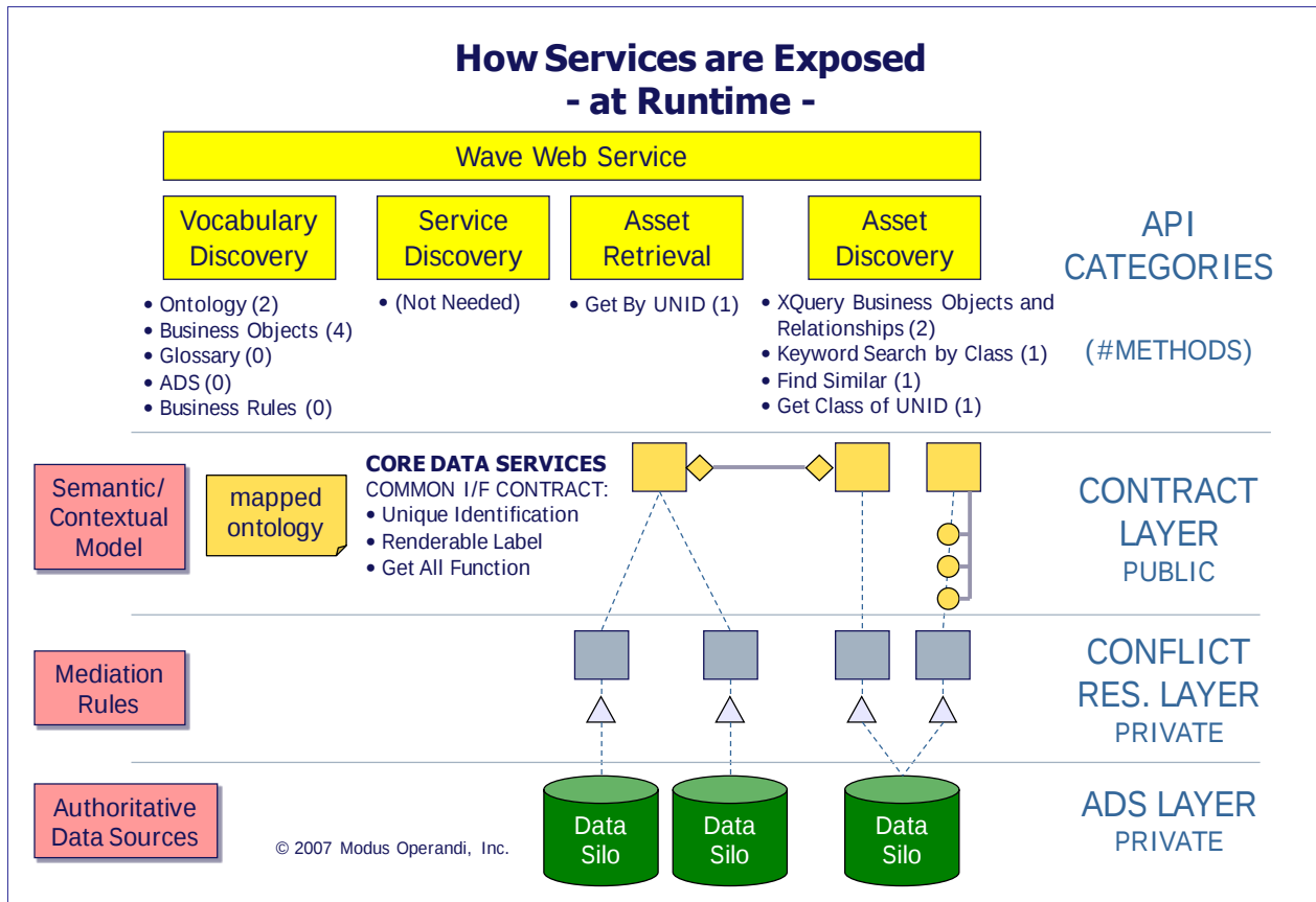
Diagram 6 – A Virtual Metadata Catalog. The mapped ontology—an OWL file—serves as a metadata repository. Metadata about instances is retrieved as needed directly from data sources.
