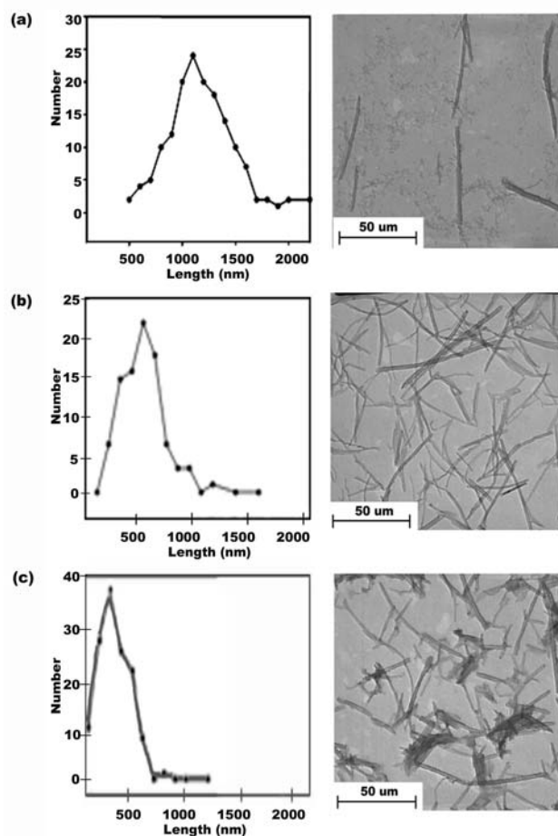
Figure 1: Sonication reduces mean length of \text{CN}_x -MWNT. \text{CN}_x -MWNT were sonicated in acid as described in Materials and Methods for 7 hours (a), 24 hours (b), and 60 hours (c). Average length was assessed by TEM.
