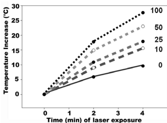
Figure 2. Effect of nanotube concentration on heating. Concentrations of nanotubes used start at 1000 \times 10^5 nanotubes/unit volume (marked as 100%). The concentration was then diluted to 500 \times 10^5 , 250 \times 10^5 , and 100 \times 10^5 nanotubes/unit volume, (marked 50%, 25% and 10% respectively). Starting temperature was approximately 23°C.
