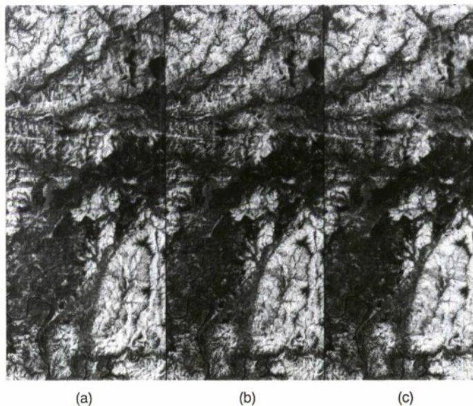
Fig. 2. TM band 4 uncorrected data (a), corrected using DEM level I (b), and corrected using DEM level II (c)
