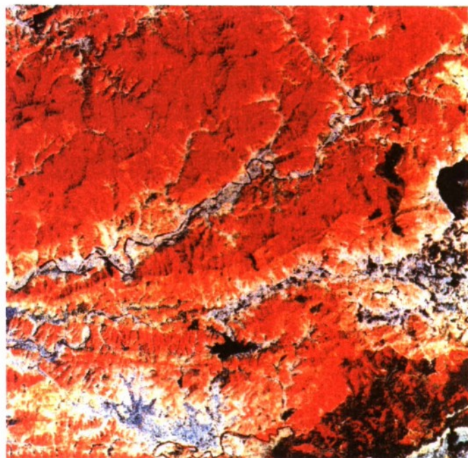
PLATE 1. Infrared composite of L3122-I 1:50,000-scale map area (50-metre resolution).
