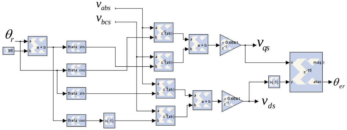
Figure 12. Stator Voltage Transformation to Rotor Reference Frame.
