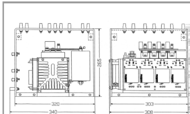
General dimensions
