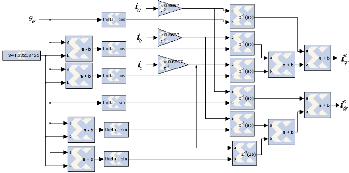
Figure 13. Rotor Current Transformations.
