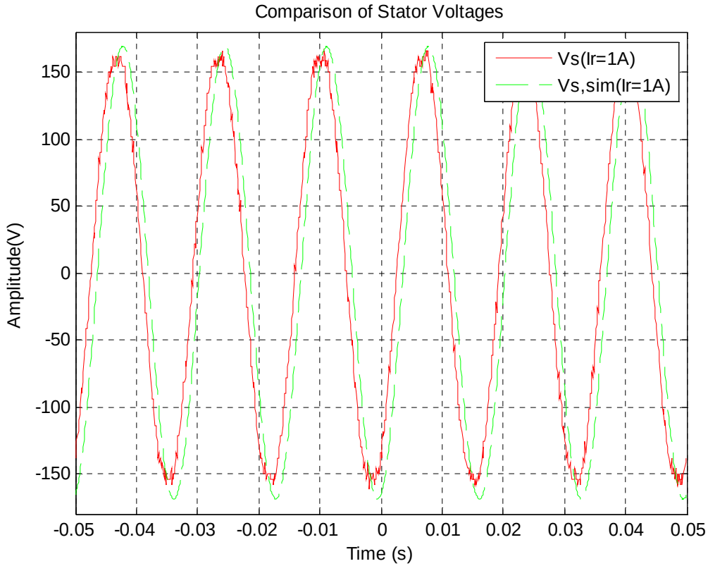
Figure 19. Comparison of Grid Stator Voltage to Simulation Source.
