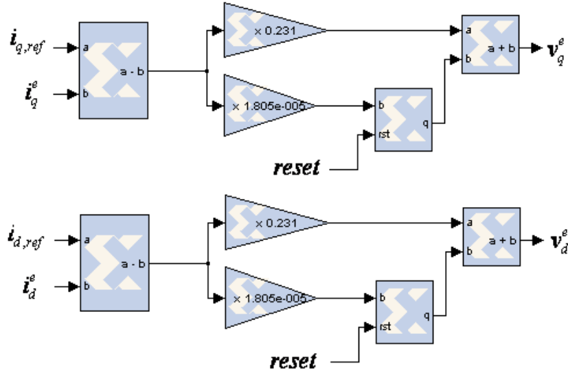
Figure 14. PI Current Controller.
