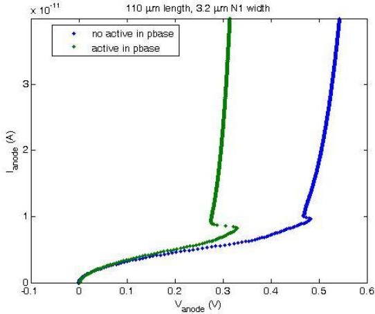
Figure 26. I-V characteristics of 3.2 \mu\text{m} N1 width SCR, 110 \mu\text{m} length.
