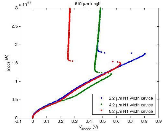
Figure 24. 510 \mu\text{m} length SCRs with different N1 widths.
