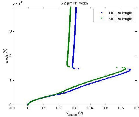
Figure 28. 5.2 μm N1 width, different lengths.
