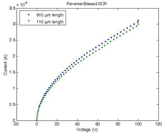
Figure 10. SCRs under reverse bias. Two devices of differing lengths are compared here, both with 5.2 \mu\text{m} N1 widths.
