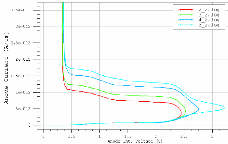
Figure 7. Moore's Atlas simulation for fabricated SCRs. (From [5]).
