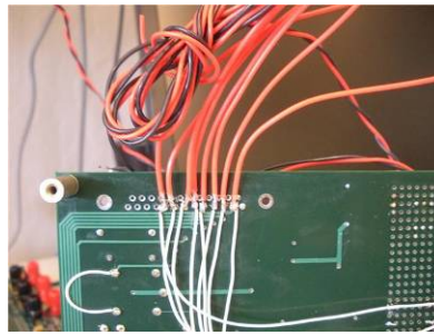
RTB 8 Connections to Prototype Board
