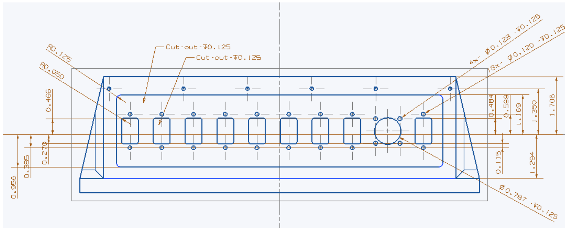
Figure 17. Final Prototype Front Face Plate Part 1
