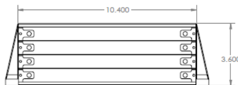
Figure 16. MIPS Front Face Plate (From DNet # 11050: Multiple Interface Payload Subsystem Envelope Drawing)
