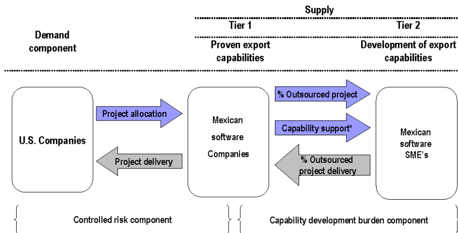
Figure 7: Acceleration Model
