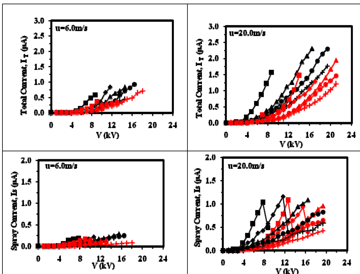
Figure 1: Total (top row) and spray (bottom row) currents for diesel oil (red) and JP-8 (black) at two different injection velocities.
