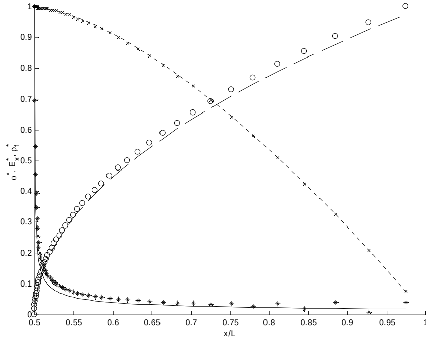
Figure 25: Analytical (lines) and numerical (symbols) to the space charge injection problem.
