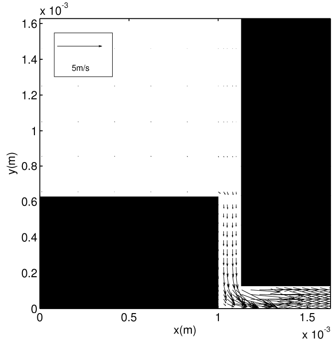
Figure 27: Velocity vectors.
