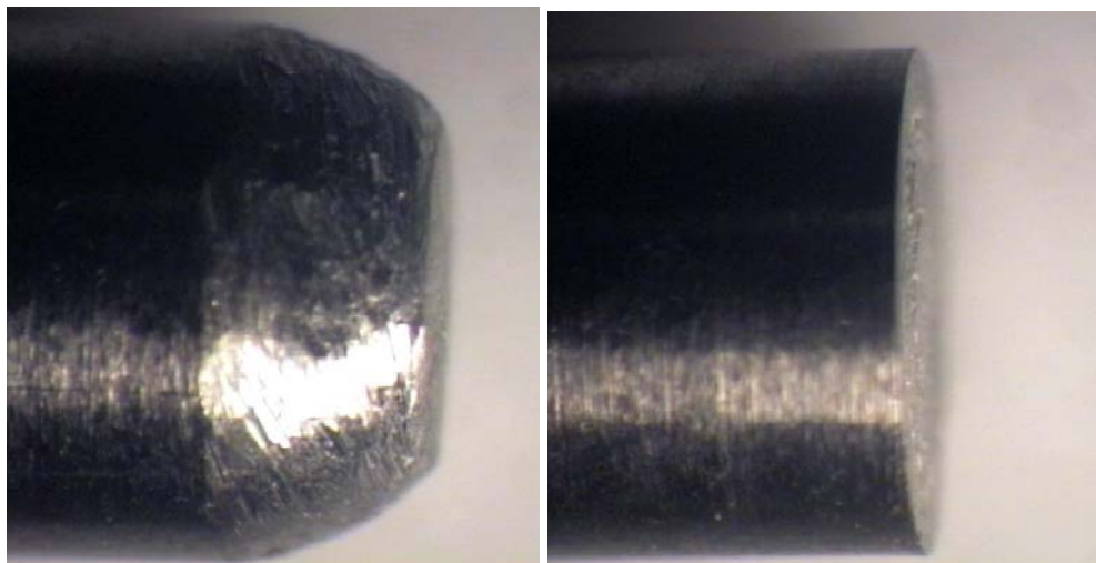
Figure A.4: Two variations of emitter surface shape of the 3 mm tungsten bar.
