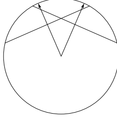
Figure 3.2: Projection of \bar{h} and \bar{h}' into the plane defined by w and w' .
