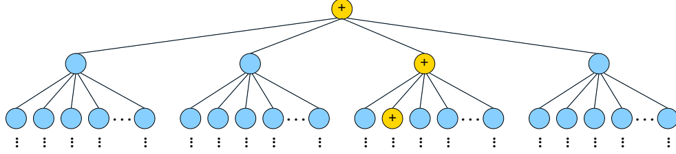
Figure 3.4: A learning problem where exponential rates are not achievable. The instance space is an infinite-depth tree. The target labels nodes along a single infinite path as +1 , and labels all other nodes -1 . For any \phi(\epsilon) = o(1/\epsilon) , when the number of children and probability mass of each node at each subsequent level are set in a certain way, label complexities of o(\phi(\epsilon)) are not achievable for all targets.
