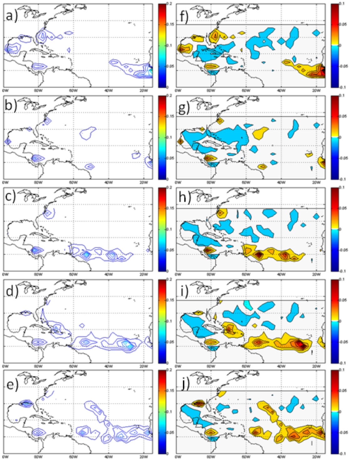
Figure 33. Seven-day summed TC formation probability forecasts (left column) and TC formation probability forecast anomalies (right column) from five forecasts initialized on 20 May 2009 and valid on: (a) 01 July 2009; (b) 8 July 2009; (c) 15 July 2009; (d) 22 July 2009; and (e) 29 July 2009. Contours start at 1 percent and are in 1 percent increments.
