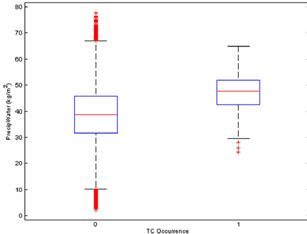
Figure 8. Box plots of precipitable water ( \text{kg/m}^2 ) grouped by whether a TC formed in a given day-grid (“0” indicates no TC formed, and “1” indicates a TC formed). The blue box encloses 50% of the precipitable water data points, the whiskers (black dashed lines) encompass ~99% of the data points. The red “+” highlight ~1% of the data points that are outliers. Produced using R2 data and TC occurrences from the HURDAT for January-December of 1982-2006.
