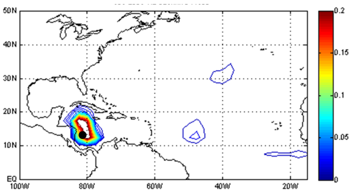
Figure 19. Zero lead seven-day summed TC formation probability hindcast centered on the 309 th day (5 November) of 2008, constructed from a 40 percent NTCI model. The black dot represents TC Paloma that formed on 5 November 2008. Contours start at 1 percent and are in 1 percent increments.
