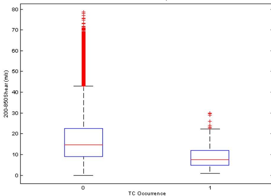
Figure 9. Box plots of 200-850mb wind shear (in m/s) grouped by whether a TC formed in a given day-grid (“0” indicates no TC formed, and “1” indicated a TC formed). The blue box encloses 50% of the wind shear data points, the whiskers (black dashed lines) encompass ~99% of the data points. The red “+” highlight ~1% of the data points that are outliers. Produced using R2 data and TC occurrences from the HURDAT for January-December of 1982-2006.
