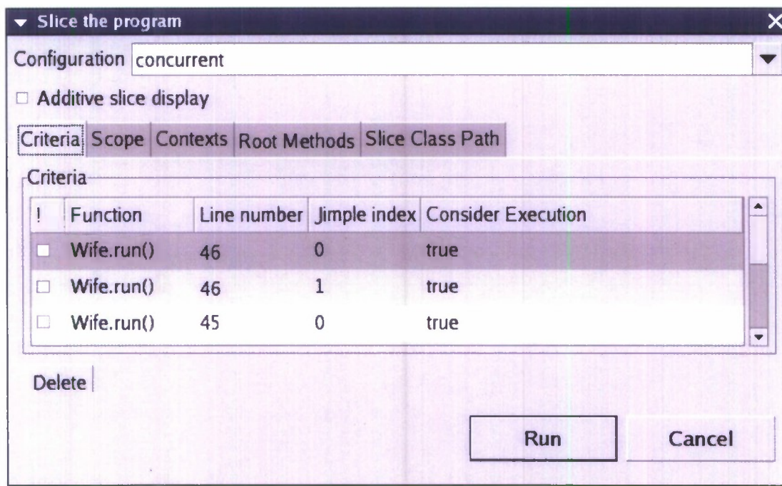
Figure 27: The Kaveri dialog that enables users to select criteria, scoping, and starting calling contexts before slicing.
