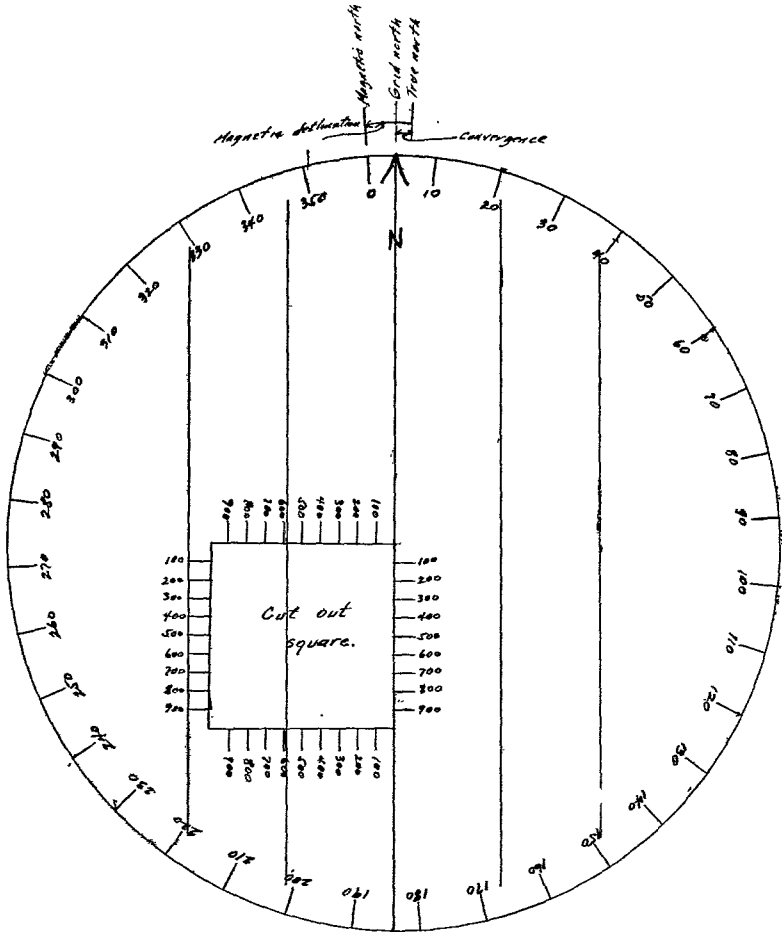
FIG 1. PLOTTING PROTRACTOR
