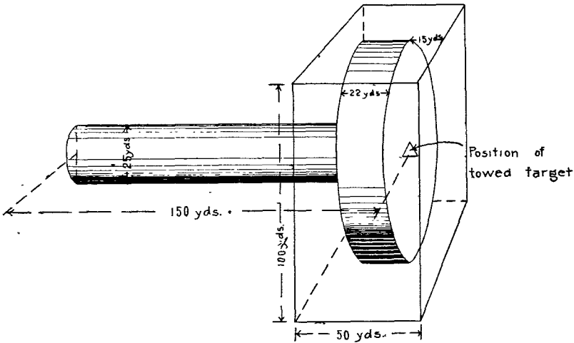
FIG. 2. NEW TARGET ENCLOSED IN THE TARGET PRESCRIBED FOR 1925
