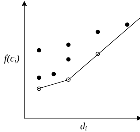
Figure 15: Convex hull of potentially optimal intervals
