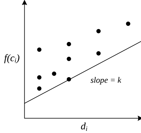
Figure 14: Interval function value versus size
