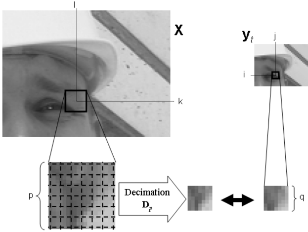
Fig. 5. Description of the expression \mathbf{D}_p \mathbf{R}_{k,l}^H \mathbf{H} \mathbf{X} - \mathbf{R}_{i,j}^L \mathbf{y}_t in (21).
