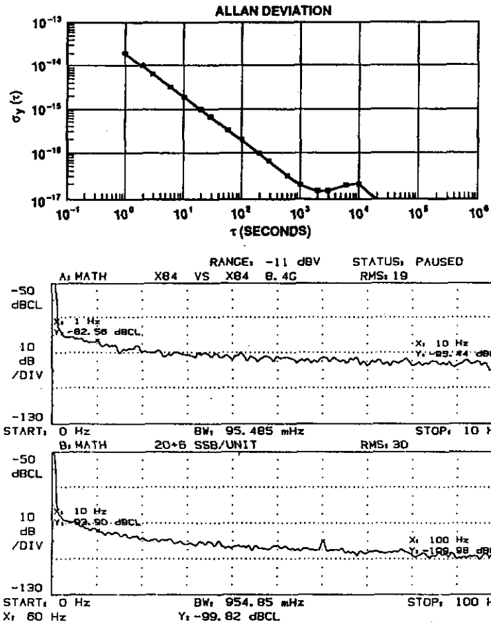
Figure 8. x 84 MULTIPLIER NOISE AT 8.4 GHz
