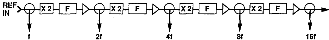
Figure 9. UNIVERSAL LOW NOISE FREQUENCY MULTIPLIER
