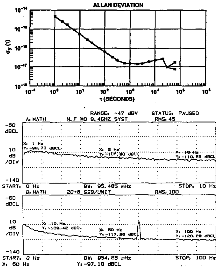
Figure 7. TEST SYSTEM NOISE FLOOR AT 8.42 GHz
