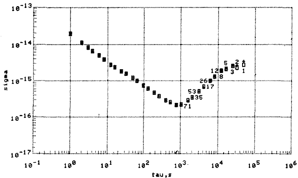
Figure 5. Experimental Allan deviation curve arising from a 3.8 km, 100 MHz passive frequency distribution system cycling 1^\circ\text{C} over a 24 hour period.
