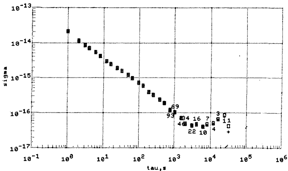
Figure 6. Experimental Allan deviation curve arising from a 3.8 km, 100 MHz actively compensating frequency distribution system consisting of a 3.8 km distribution cable (cycling 1^\circ\text{C} over 24 hours) stabilized by a 200 m coil under thermal electric control.
