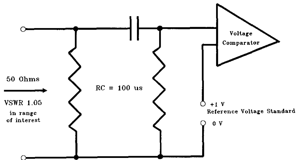
Example of Standard 1PPS Input Circuit Figure 3.
