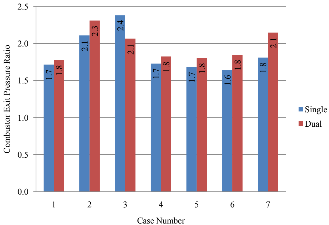
Figure 23: Combustor exit pressure ratios
