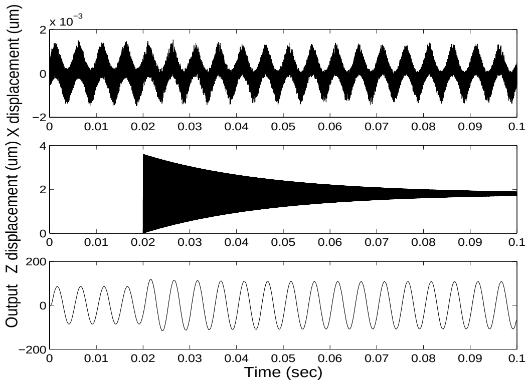
Figure 6-16: Proof-mass displacement in x and z axes and modulator output of the 2nd-order 1-bit modulator at 1000 g z-axis step input. The Q is 1000 in both axes.
