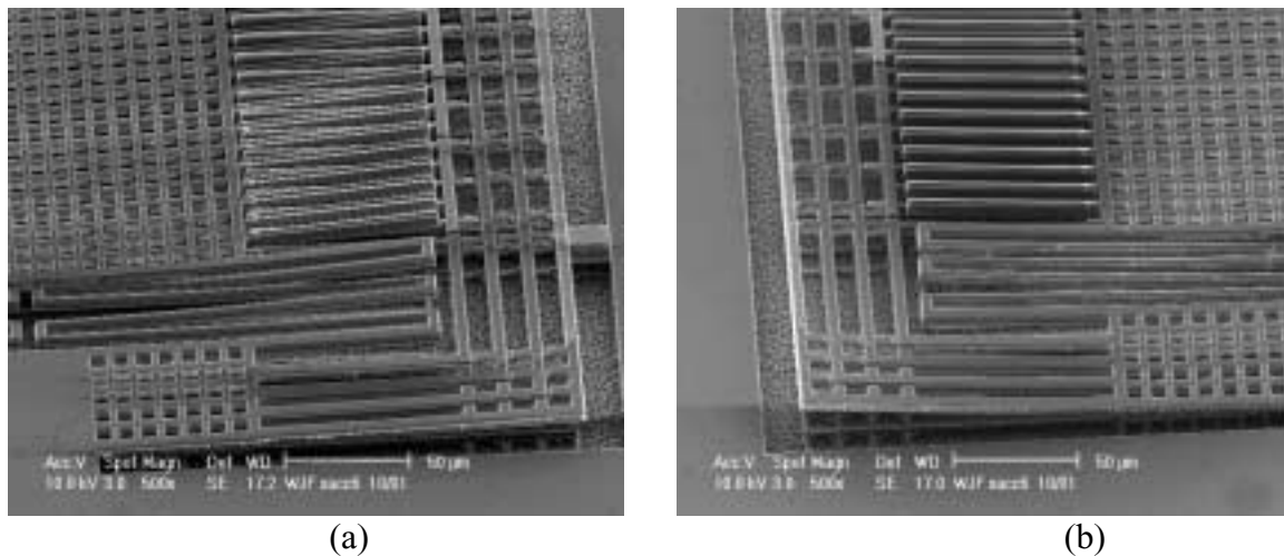
Figure 2-5: Finger mismatches without (a) and with (b) curling matching frame.
