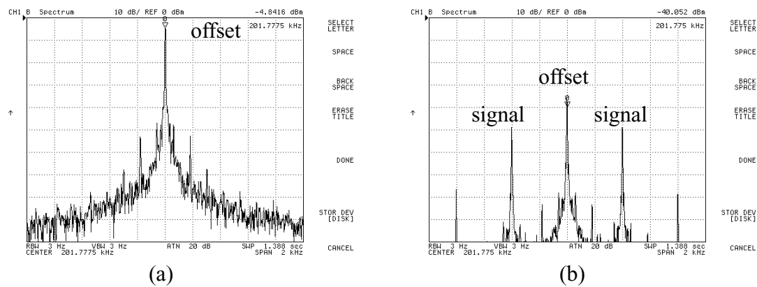
Figure 4-32: Spectrum of pre-demodulation signals: (a) the signal is blocked by ac sensor offset greater than 100 g; (b) signal appears after the sensor offset is reduced by 40 dB.
