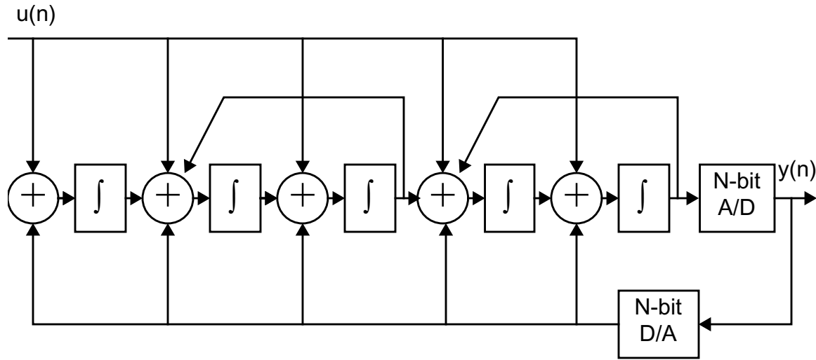
Figure 5-9: Interpolative high-order \Delta - \Sigma modulator.
