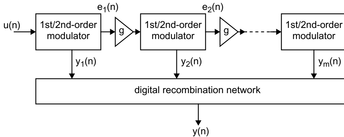
Figure 5-10: Cascade high-order \Delta - \Sigma modulator with multi-stage noise shaping (MASH).
