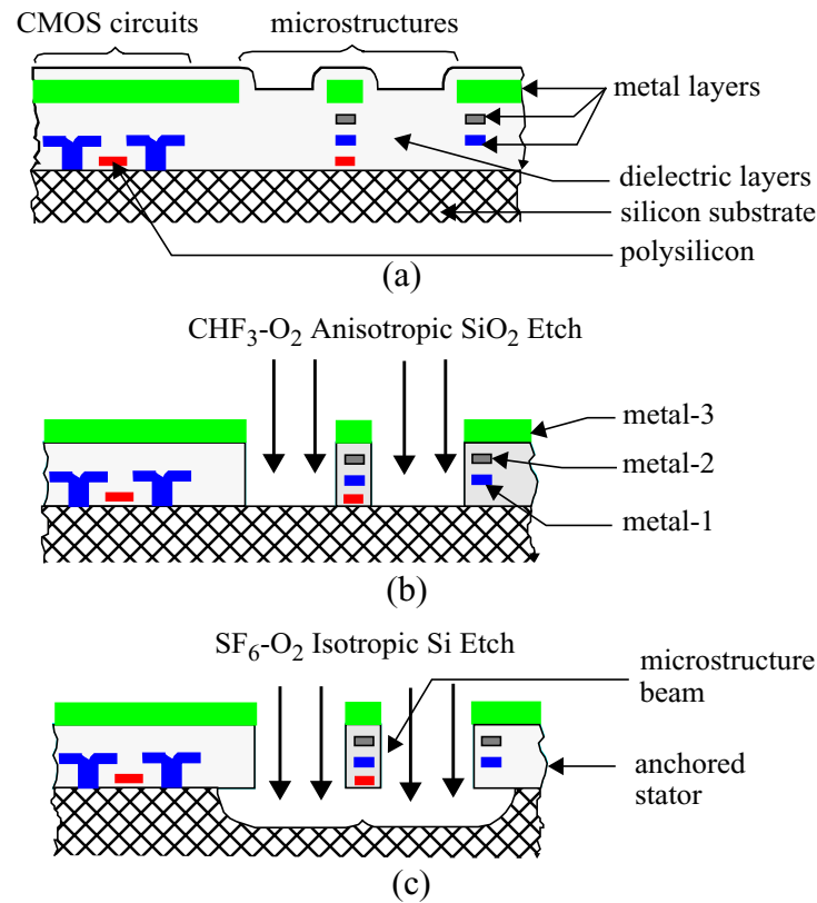
Figure 2-1: Process flow of CMOS MEMS surface micromachining.
