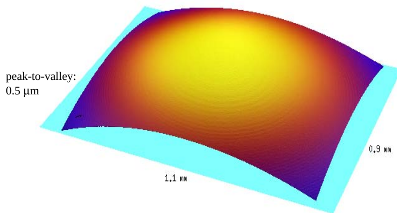
Figure 4-6: Contour plot of the electrostatic mirror profile.
