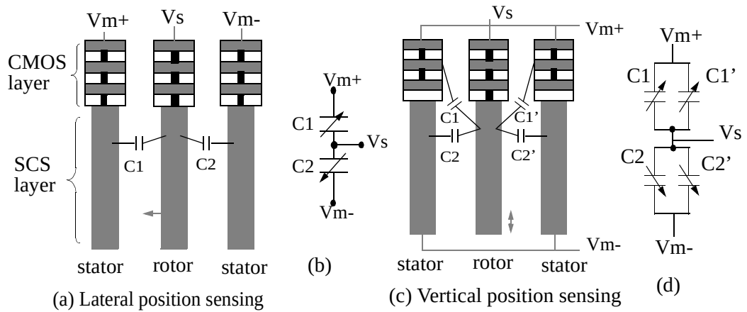
Figure 3-20: Cross-sections and wiring configurations of comb fingers for 3D vibration detection.
