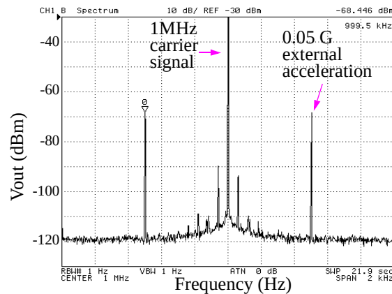
Figure 6-6: Spectrum of the y-axis accelerometer at a 500 Hz, 0.05 G external acceleration, showing a resolution of 100 \mu\text{G}/\text{Hz}^{1/2} .
