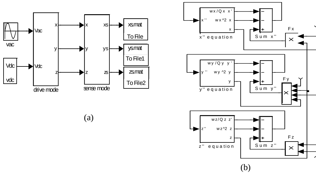
Figure 5-8: Matlab/Simulink model for a 3D comb drive. (a) Top cell. (b) Sub-cell for the drive mode.
