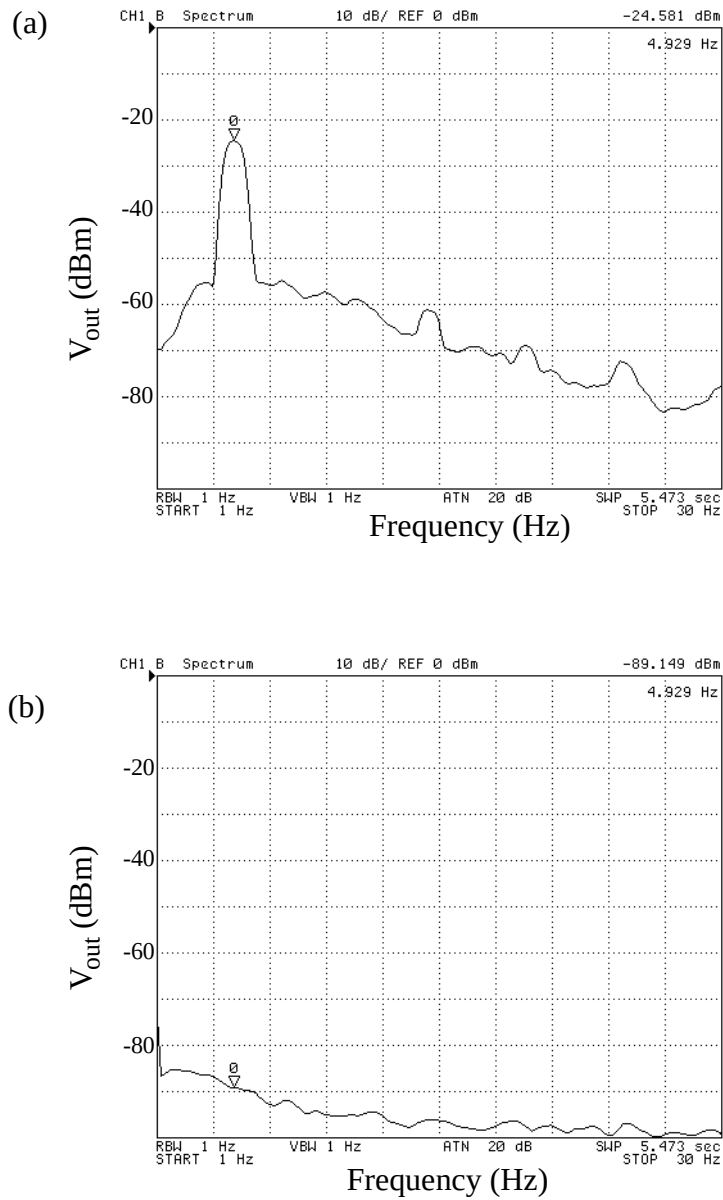
Figure 6-28: Spectrum of the output signal. (a) At 5 Hz 33°/s rotation. (b) At zero rotation.
