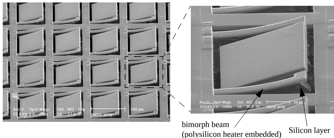
Figure 4-17: Micromirror array. Mirror size: 60 \mu\text{m} \times 60 \mu\text{m} .
