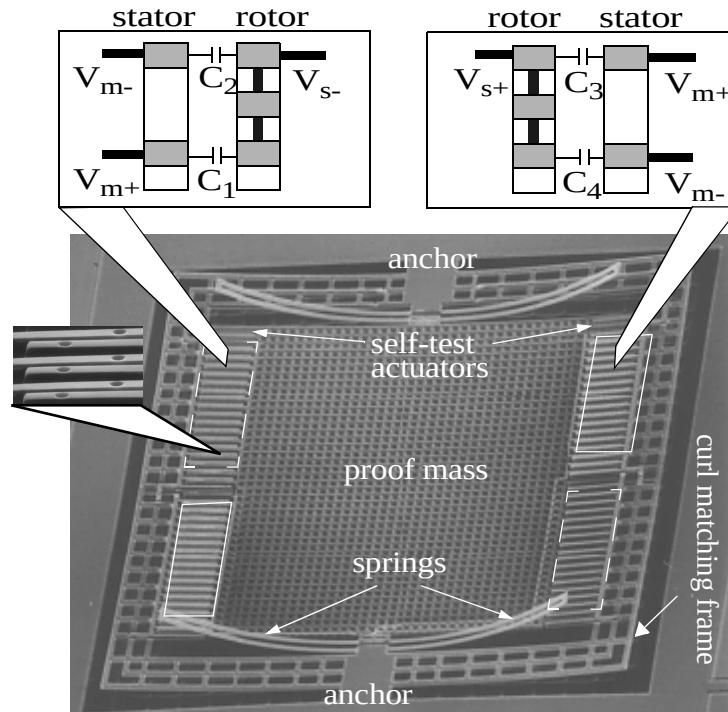
Figure 3-9: Top view of a released z-axis accelerometer.
