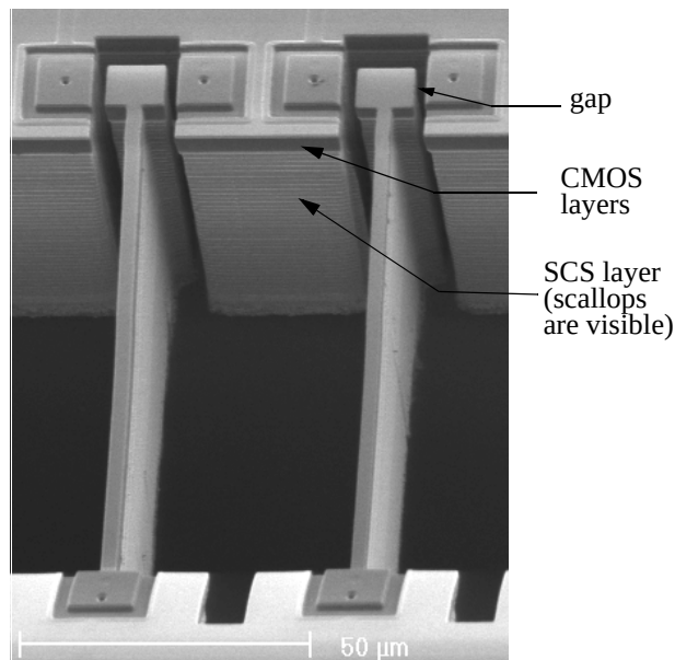
Figure 2-12: SEM of DRIE cantilever beam resonators.
