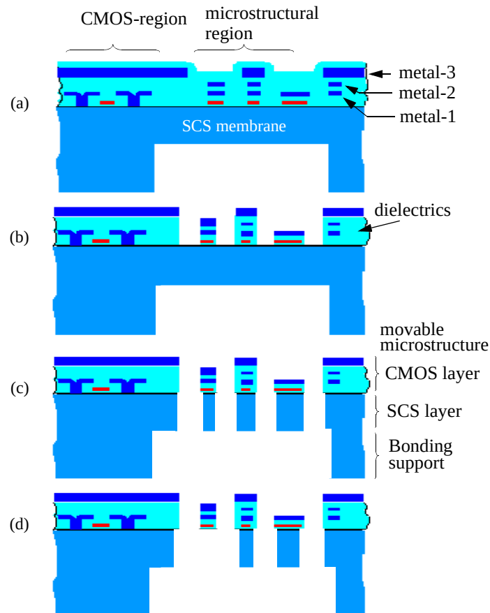
Figure 2-5: The process-flow for DRIE CMOS micromachining. (a) CMOS-chip with backside etch. (b) Anisotropic dielectric etch. (c) Anisotropic silicon etch for release. (d) An optional, short isotropic silicon etch for undercut control.
