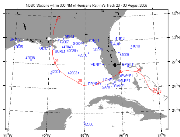
Figure 1. NDBC Stations within 300 Nautical Miles of Hurricane Katrina's Track
