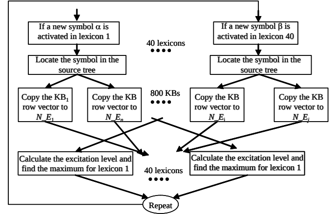
Figure 8 Flow diagram of the recall function
