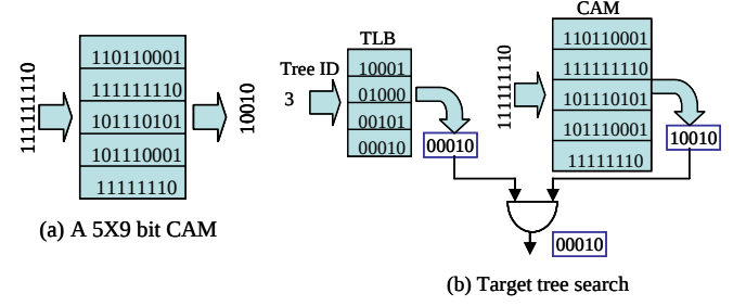
Figure 9 CAM and TLB
